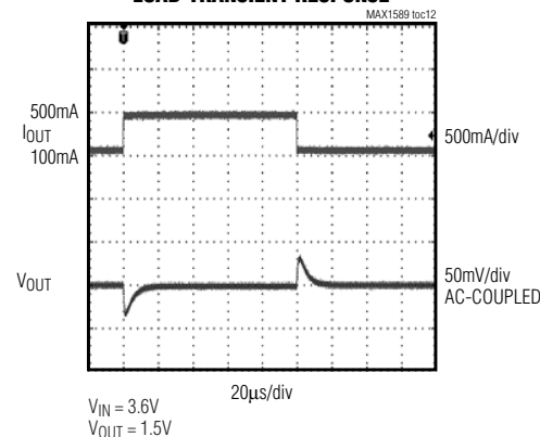
LOAD-TRANSIENT RESPONSE
