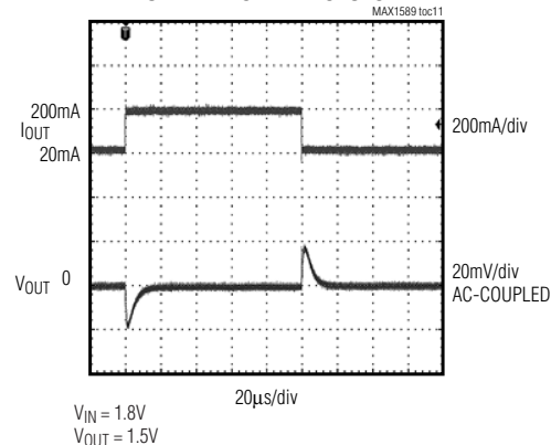
LOAD-TRANSIENT RESPONSE
