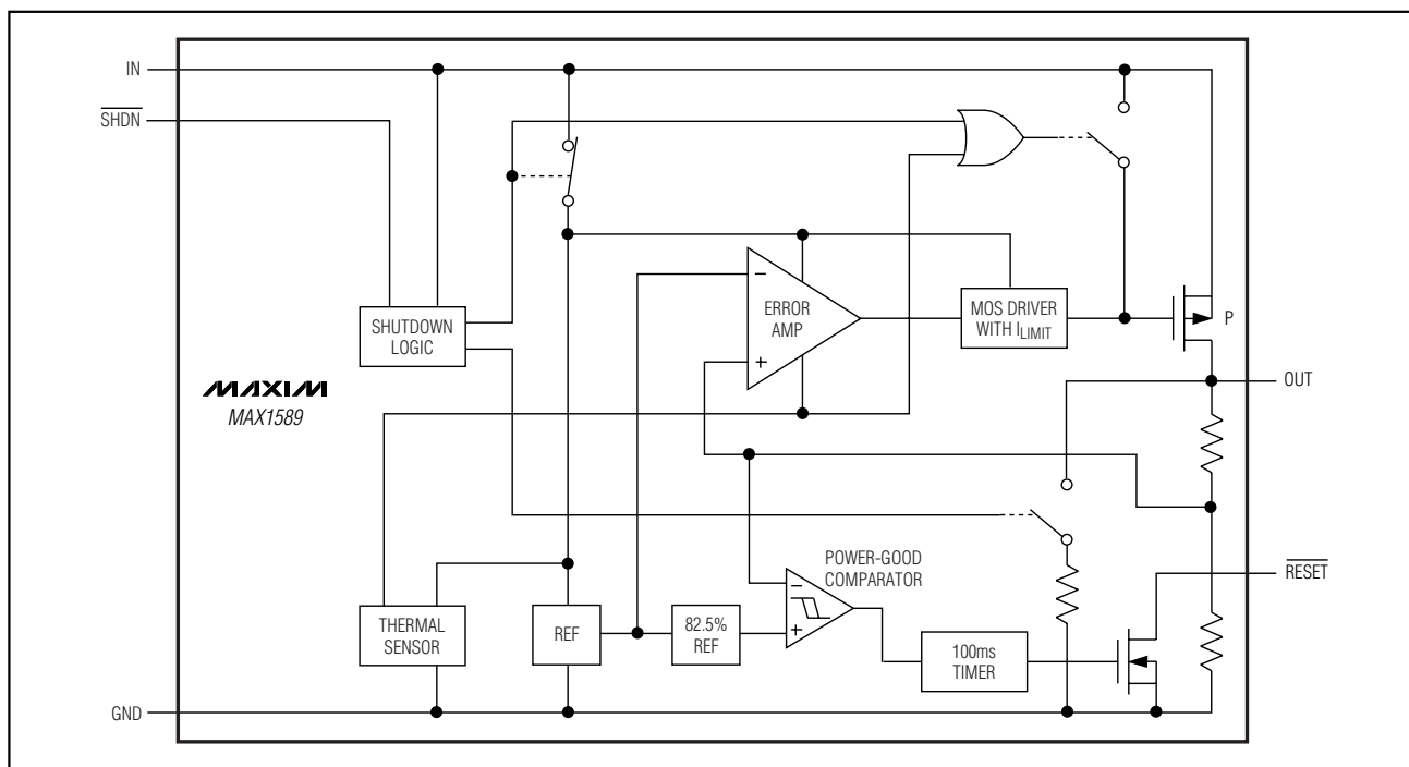
Figure 1. Functional Diagram
