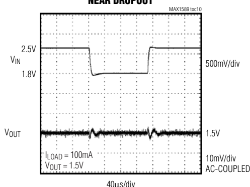
LINE-TRANSIENT RESPONSE NEAR DROPOUT
