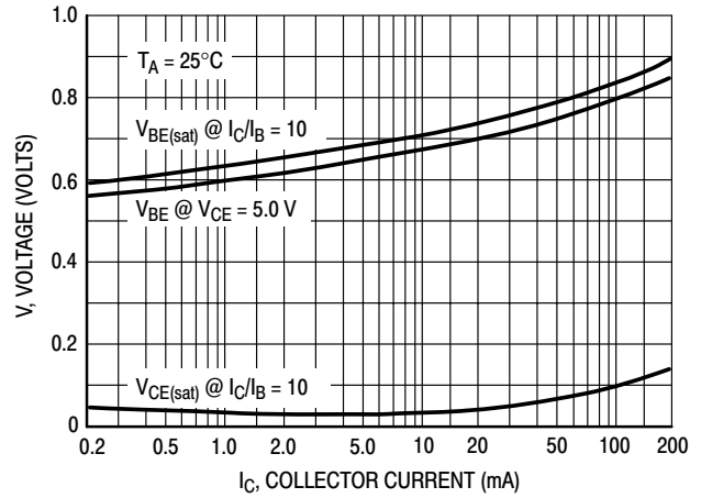
Figure 8. "On" Voltage
