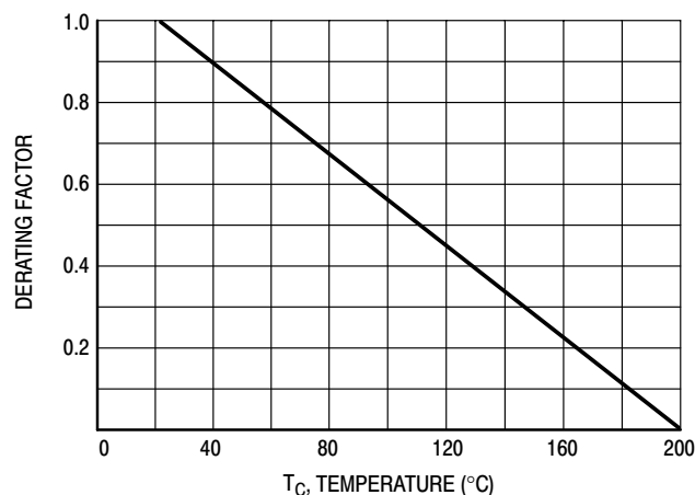
Figure 1. Power Derating
