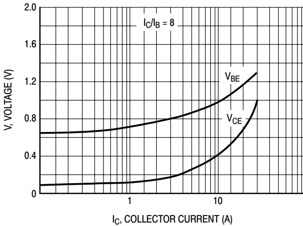
Figure 3. "On" Voltages
