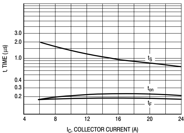
Figure 5. Resistive Switching Performance
