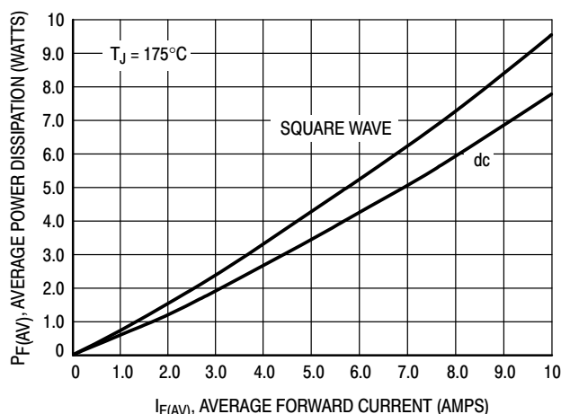
Figure 5. Power Dissipation
