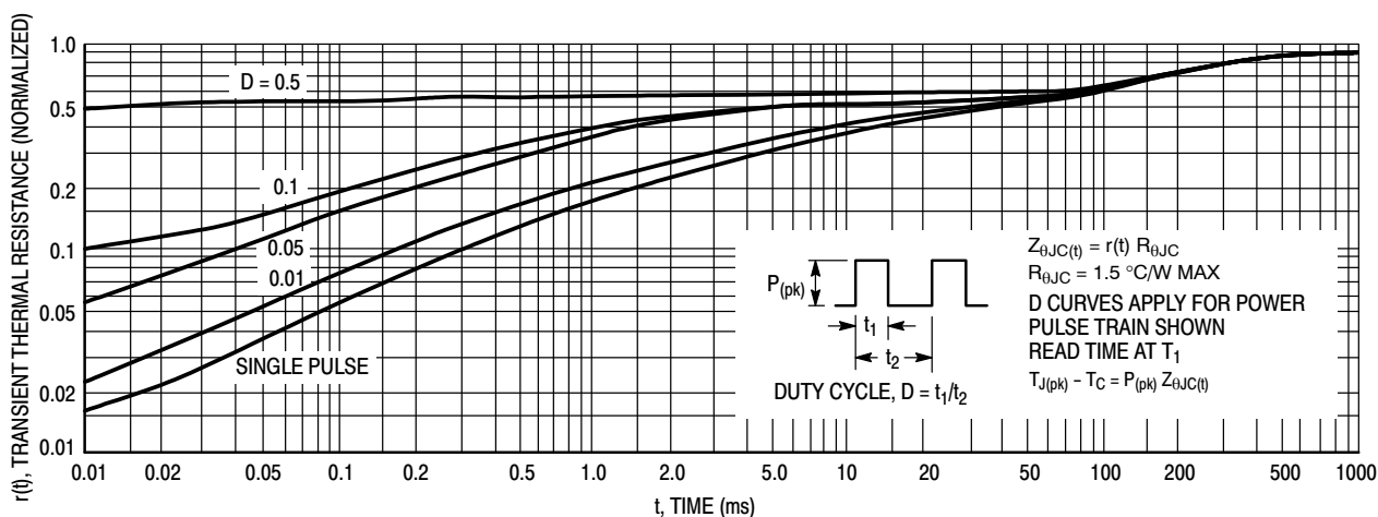
Figure 6. Thermal Response
