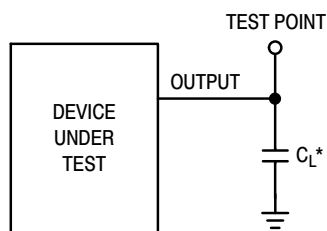
Figure 4. Propagation Delay Test Circuit
