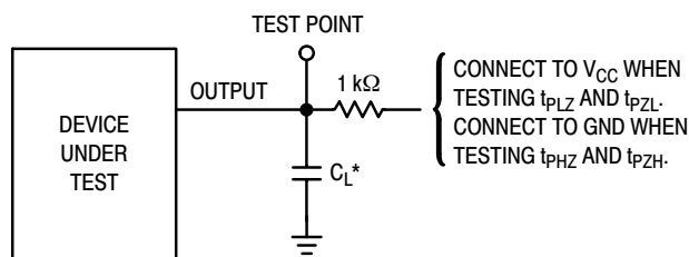
Figure 5. Three-State Test Circuit
