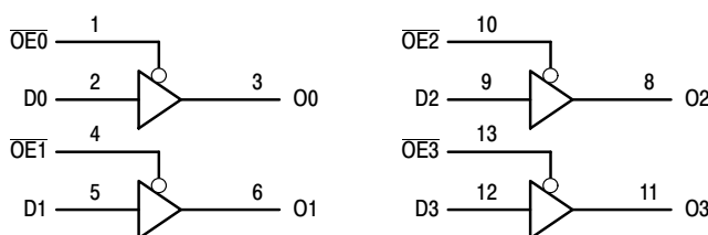
Figure 1. Logic Diagram
