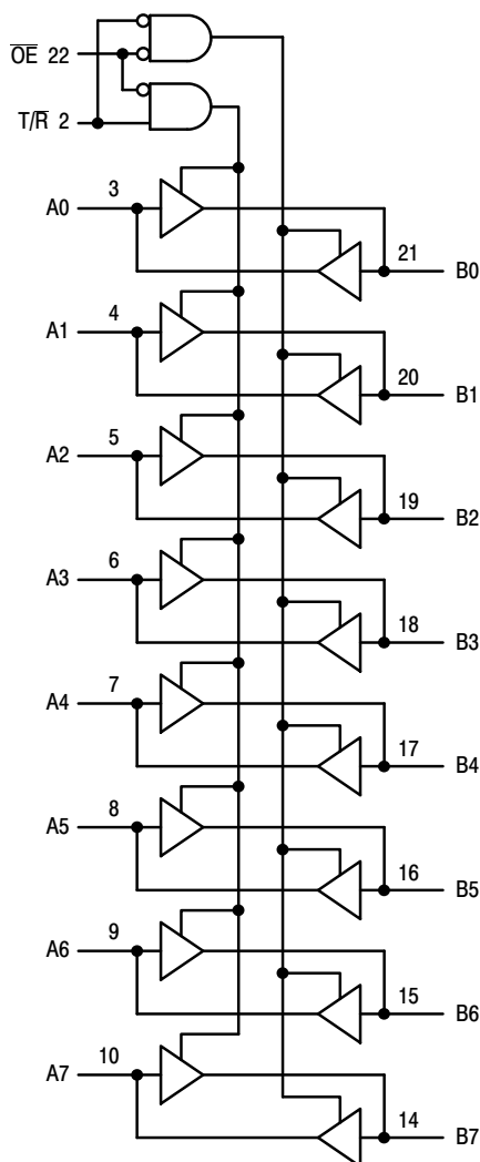
Figure 2. Logic Diagram
