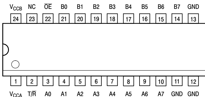
Figure 1. 24-Lead Pinout (Top View)
