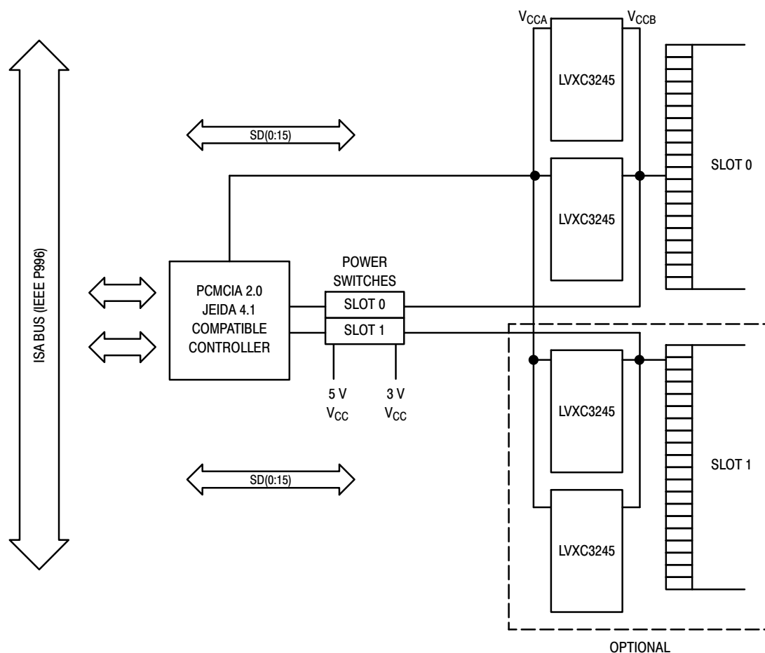
Figure 3. Block Diagram
