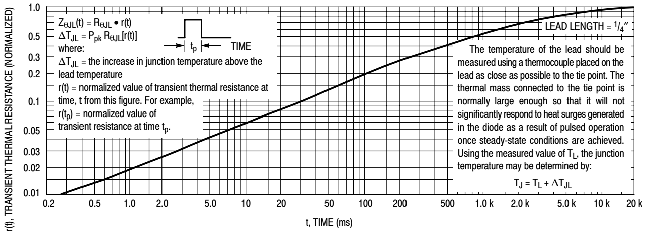
Figure 5. Thermal Response
