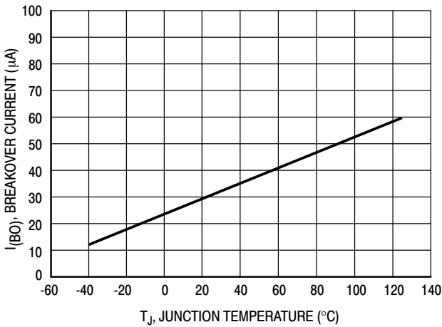
Figure 6. Typical Breakover Current
