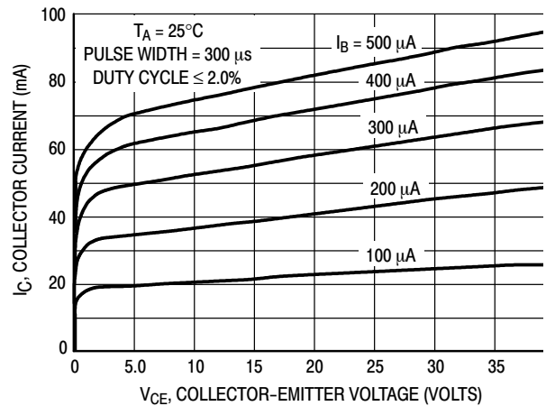
Figure 10. Collector Characteristics
