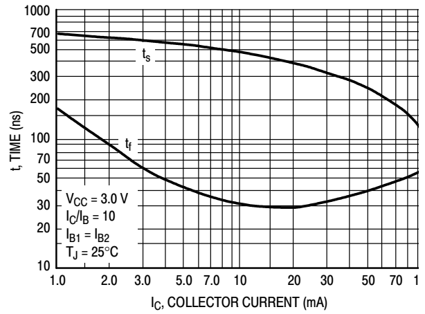
Figure 14. Turn-Off Time
