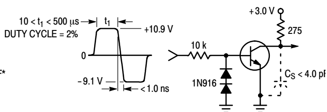
Figure 2. Turn-Off Time
