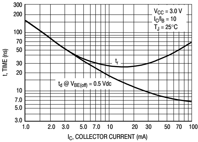
Figure 13. Turn-On Time
