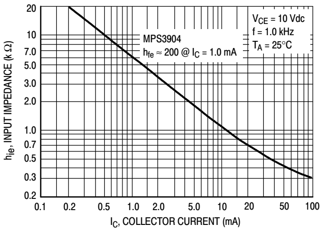
Figure 17. Input Impedance
