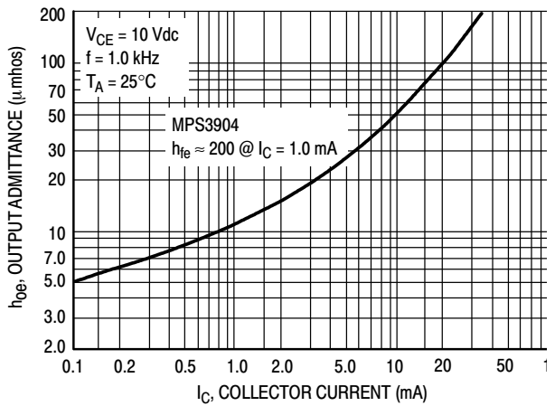
Figure 18. Output Admittance
