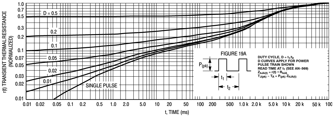
Figure 19. Thermal Response
