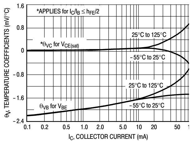
Figure 12. Temperature Coefficients
