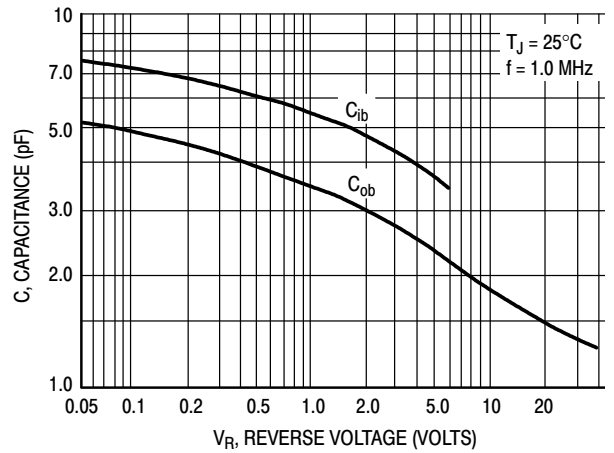
Figure 16. Capacitance
