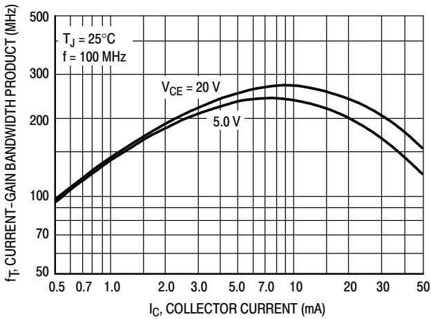
Figure 15. Current-Gain — Bandwidth Product
