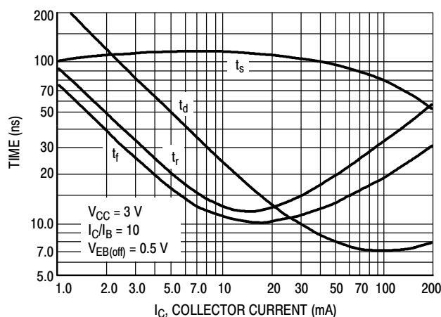
Figure 2. Switching Times
