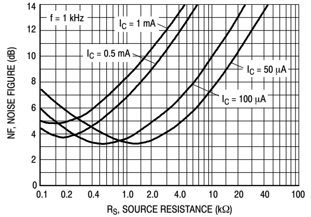
Figure 4. Source Resistance
