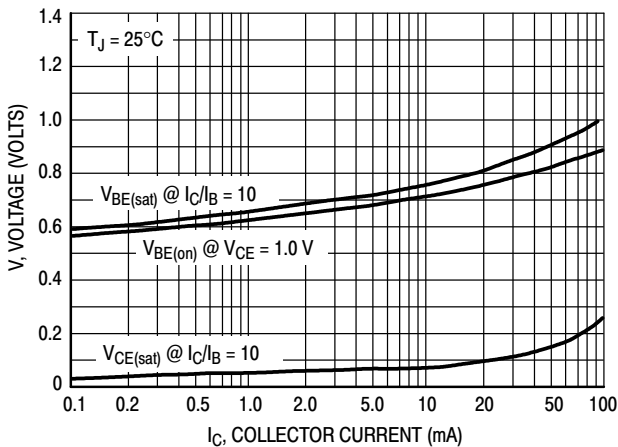
Figure 9. "On" Voltages
