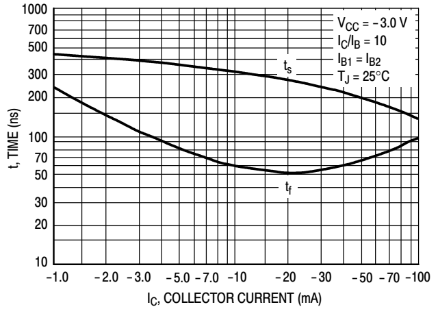
Figure 12. Turn-Off Time
