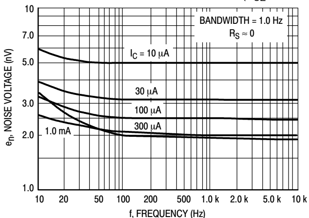
Figure 1. Noise Voltage
