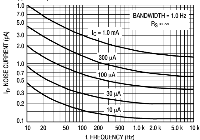
Figure 2. Noise Current
