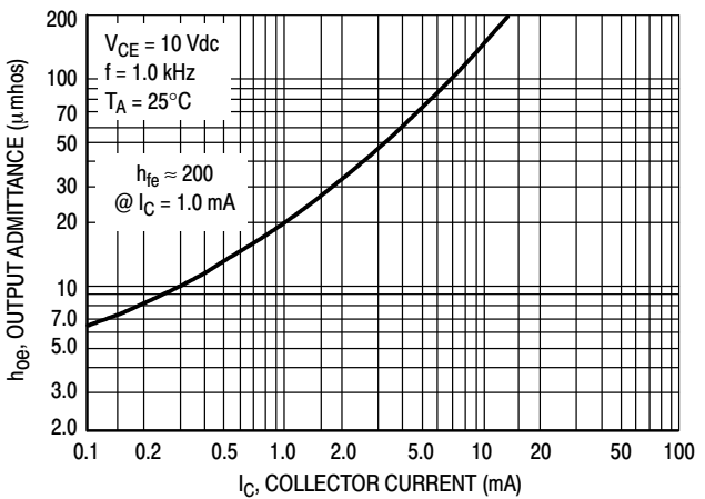
Figure 16. Output Admittance
