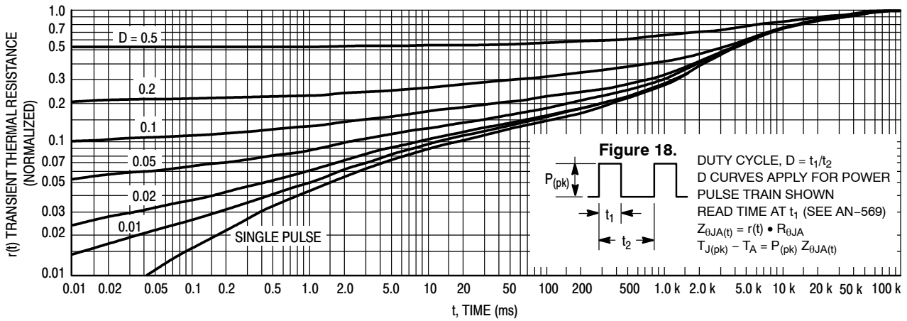
Figure 17. Thermal Response
