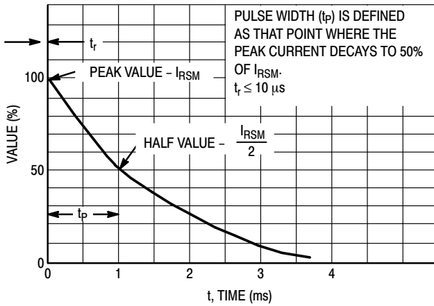
Figure 5. 10 × 1000 μs Pulse Waveform
