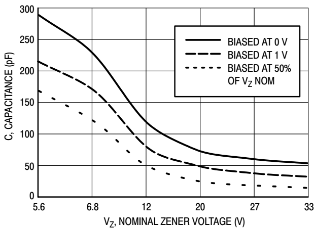
Figure 1. Typical Capacitance
