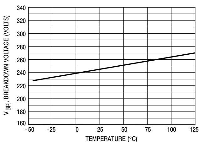
Figure 2. Breakdown Voltage versus Temperature
