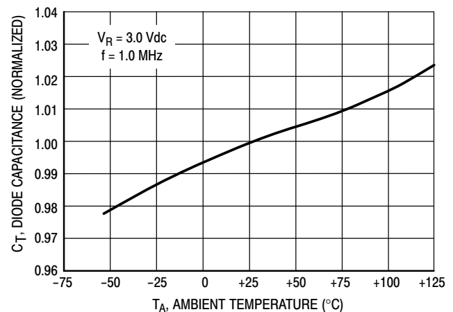
Figure 4. Diode Capacitance
