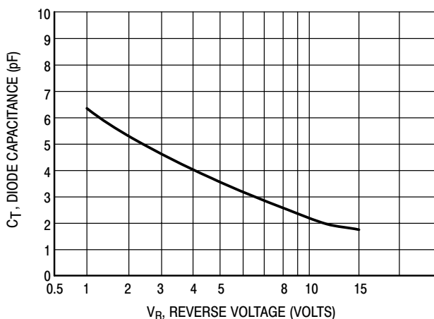
Figure 1. Diode Capacitance
