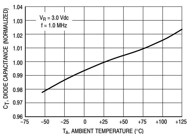
Figure 4. Diode Capacitance
