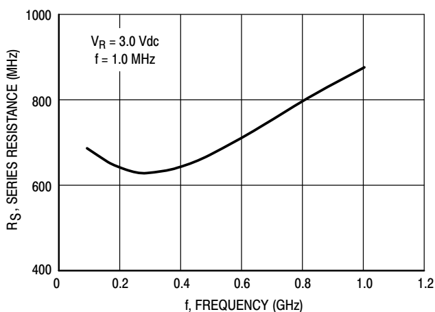
Figure 3. Series Resistance
