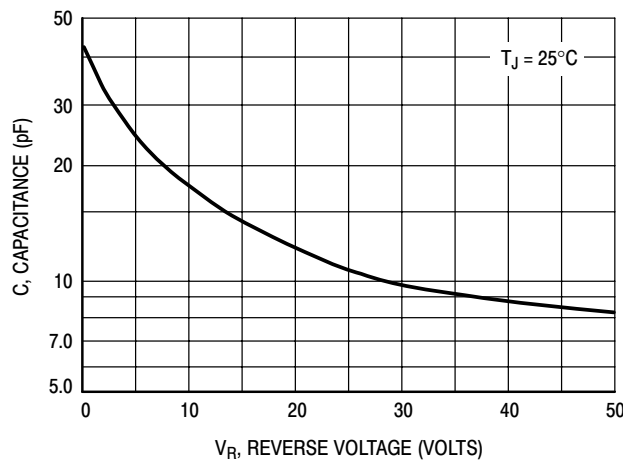
Figure 7. Typical Capacitance
