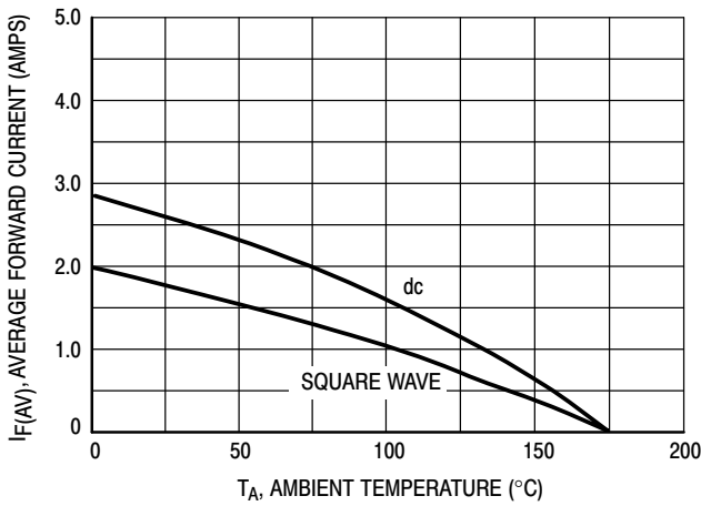
Figure 5. Current Derating
