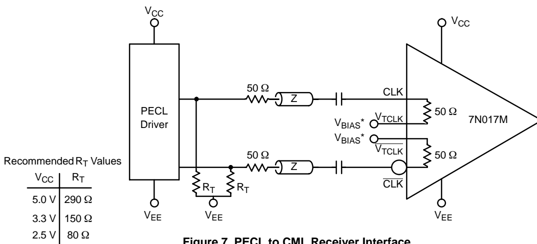
Figure 7. PECL to CML Receiver Interface
