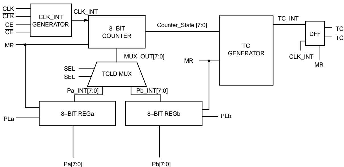
Figure 4. Block Diagram
