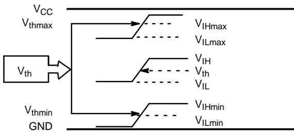
Figure 21. V_{th} Diagram
