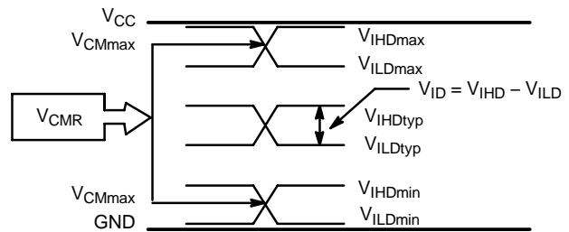
Figure 22. V_{CMR} Diagram
