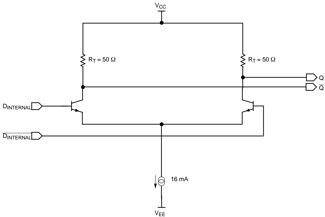
Figure 3. Output Structure
