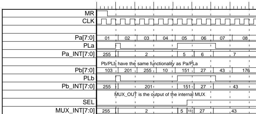
Figure 17. Timing Diagram Relating PLa, PLb, Pa(0:7), Pb(0:7)
