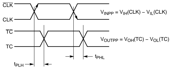
Figure 18. AC Reference Measurement
