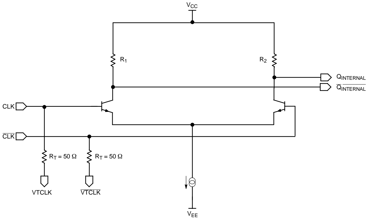
Figure 2. Input Structure
