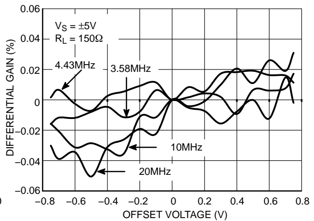
Figure 16. Differential Gain
