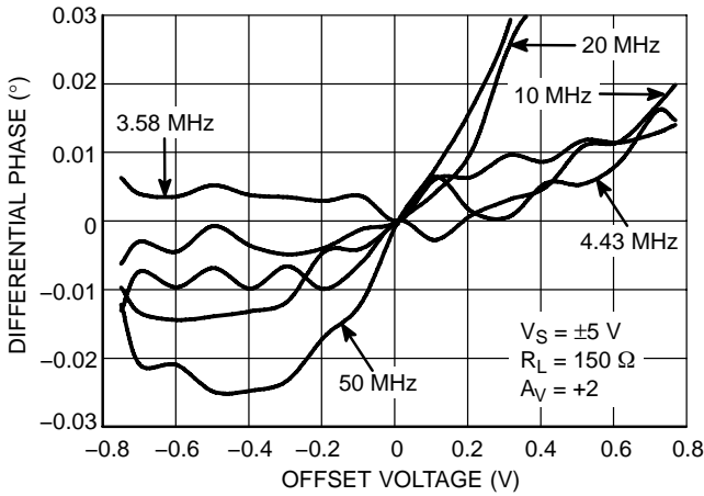
Figure 17. Differential Phase
