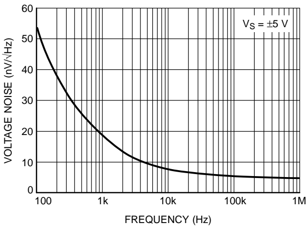
Figure 13. Input Referred Voltage Noise vs. Frequency
