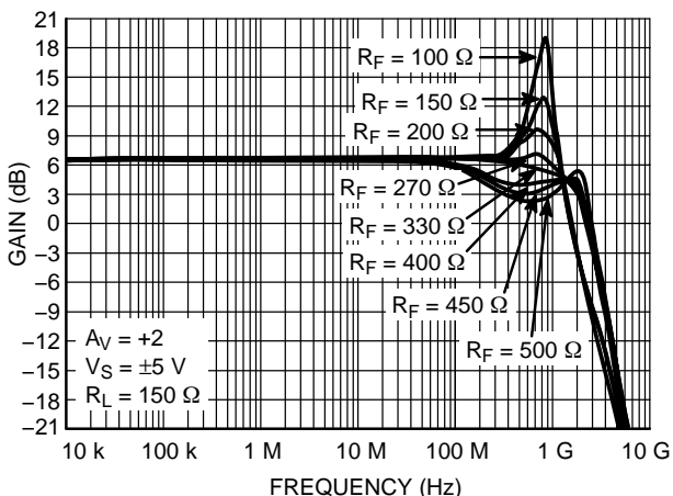
Figure 23. Frequency Response vs. R_F
