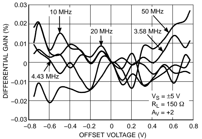
Figure 16. Differential Gain
