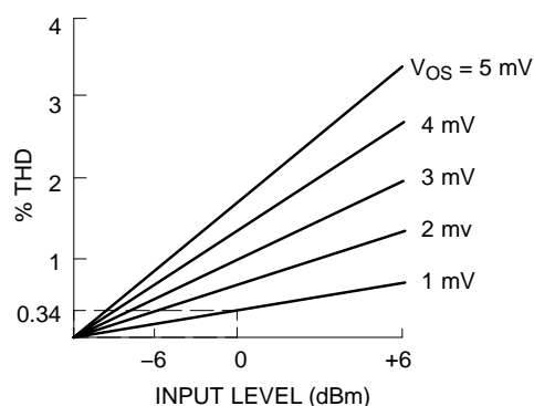
Figure 13. ΔG Cell Distortion vs. Offset Voltage
