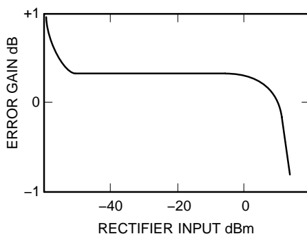
Figure 10. Rectifier Accuracy
