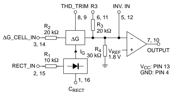
Figure 5. Chip Block Diagram (1 of 2 Channels)
