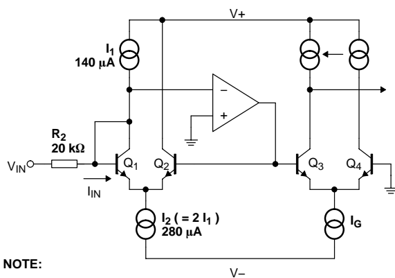
Figure 12. Simplified ΔG Cell Schematic
