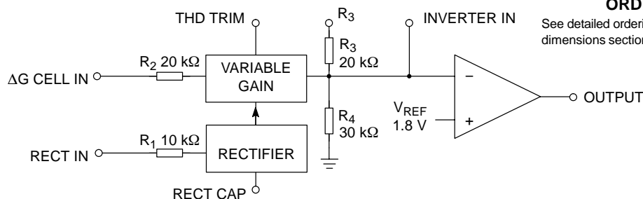
Figure 1. Block Diagram
