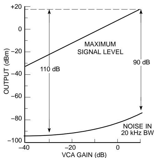
Figure 15. Dynamic Range
