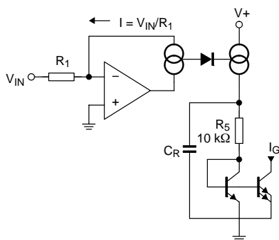
Figure 8. Rectifier Concept
