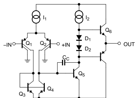
Figure 17. Operational Amplifier
