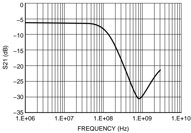
Figure 1. Insertion Loss Characteristic (50 Ω Source and 50 Ω Load Termination)
