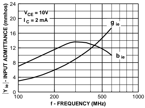
Input Admittance
