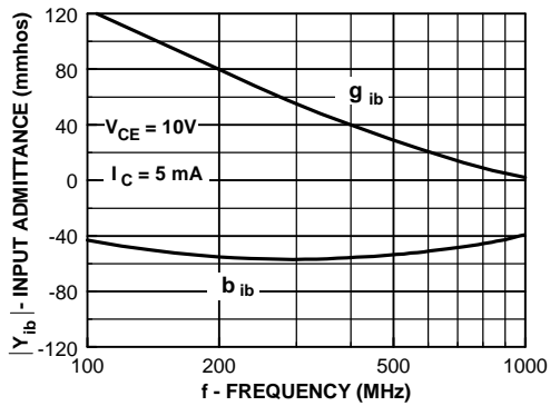
Input Admittance
