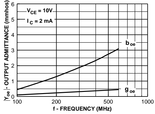
Output Admittance
