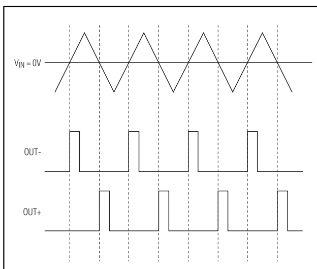
Figure 1. MAX9714 Outputs with No Input Signal Applied
