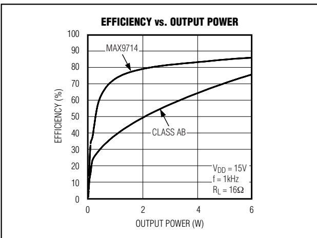
Figure 3. MAX9714 Efficiency vs. Class AB Efficiency
