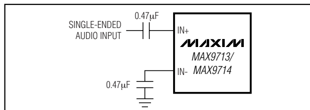
Figure 5. Single-Ended Input
