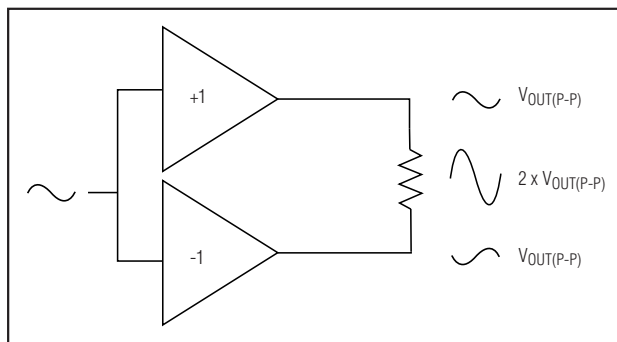
Figure 1. Bridge-Tied Load Configuration
