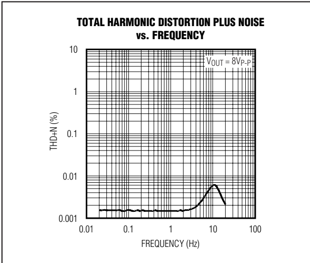
Figure 2. MAX9711 Piezoelectric Speaker Driver THD+N vs. Frequency
