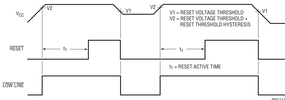
Figure 1. Reset Active Time
