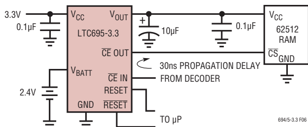
Figure 6. A Typical Nonvolatile CMOS RAM Application
