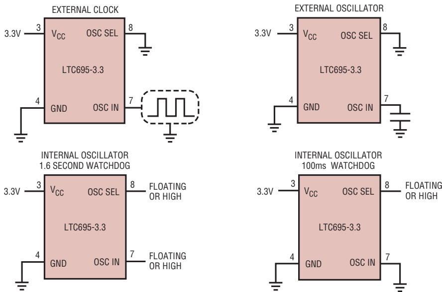
Figure 12. Oscillator Configurations
