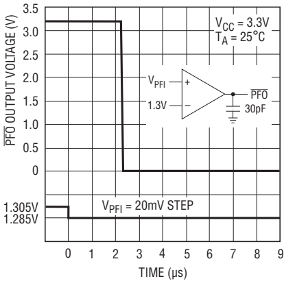
Power-Fail Comparator Response Time
