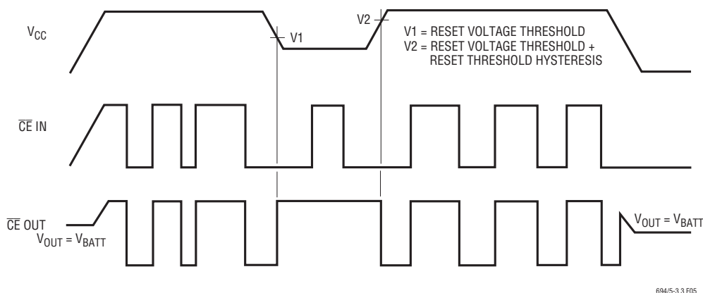
Figure 5. Timing Diagram for \overline{\text{CE}} \text{ IN} and \overline{\text{CE}} \text{ OUT}
