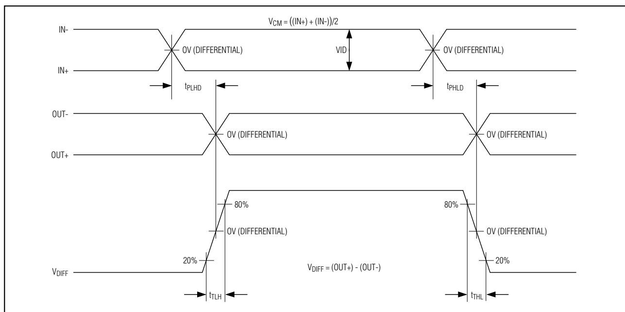
Figure 4. Transition Time and Propagation Delay Timing Diagram
