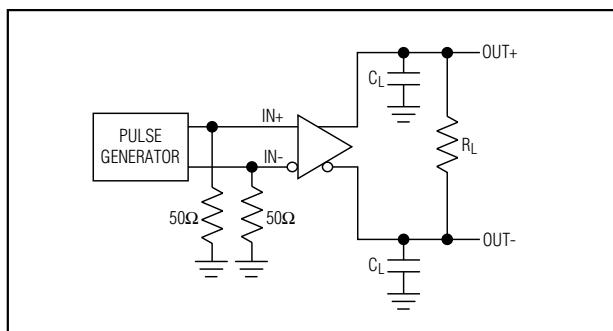
Figure 3. Transition Time and Propagation Delay Test Circuit
