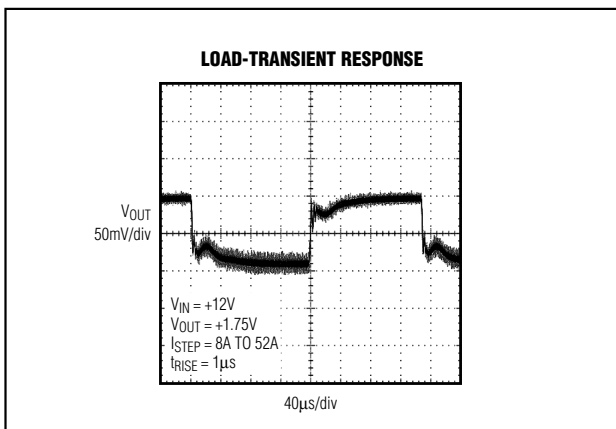
Figure 8. MAX5037 EV Kit Transient Response
