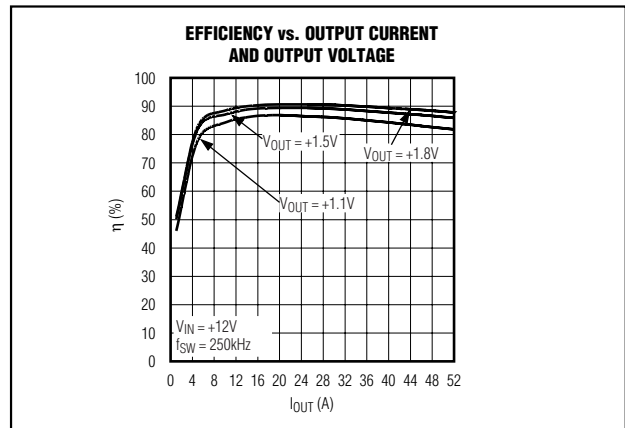
Figure 10. Efficiency vs. Output Current and Output Voltage
