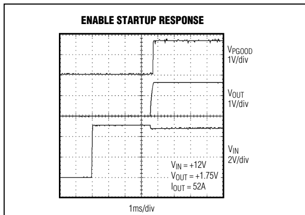
Figure 14. Enable Startup Response
