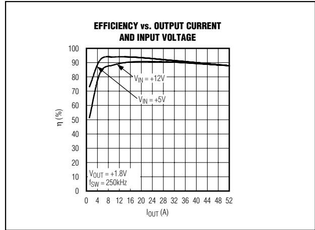
Figure 9. Efficiency vs. Output Current and Input Voltage
