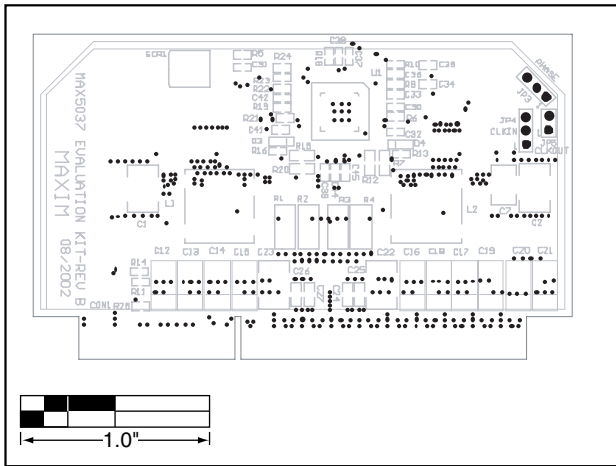
Figure 19. MAX5037 EV Kit Component Placement Guide—Component Side
