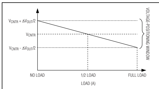
Figure 2. VRM Loadline with V_{CNTR} = VID at Half Load
