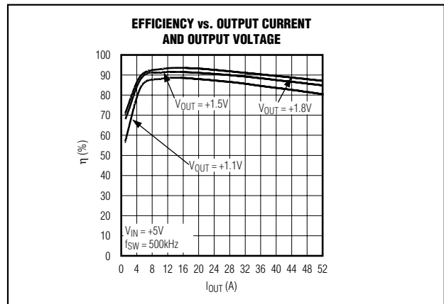
Figure 11. Efficiency vs. Output Current and Output Voltage
