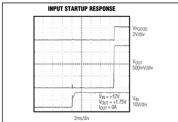
Figure 12. Input Startup Response
