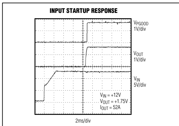
Figure 13. Input Startup Response
