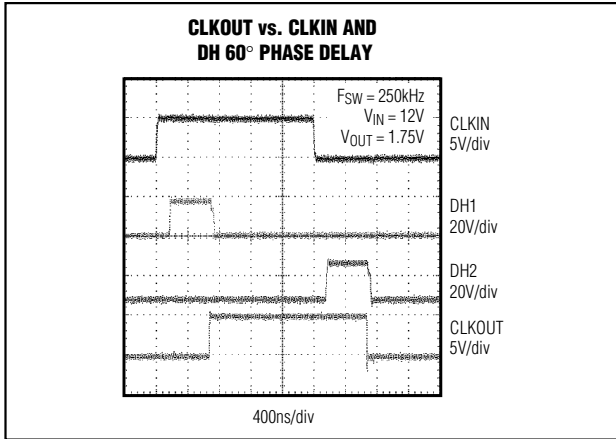
Figure 15. CLKOUT vs. CLKIN and DH 60° Phase Delay
