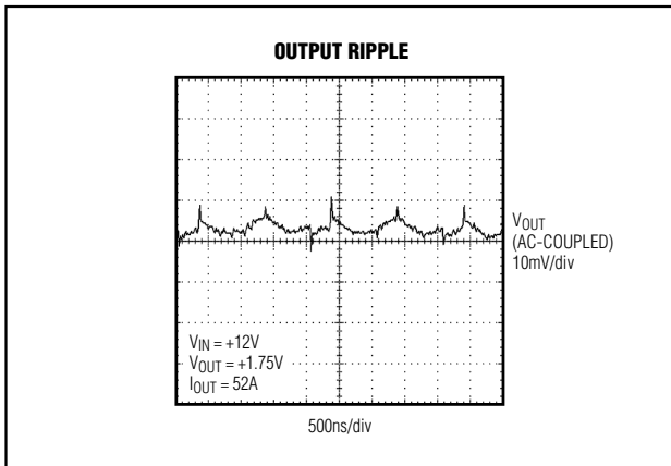
Figure 7. Output Ripple
