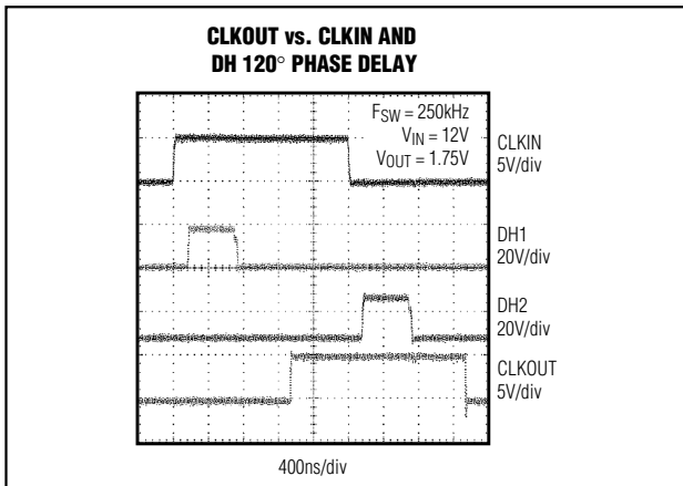
Figure 17. CLKOUT vs. CLKIN and DH 120° Phase Delay
