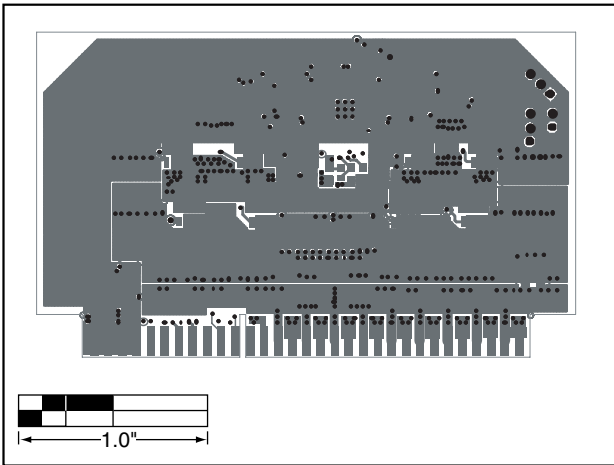
Figure 23. MAX5037 EV Kit PC Board Layout—Solder Side
