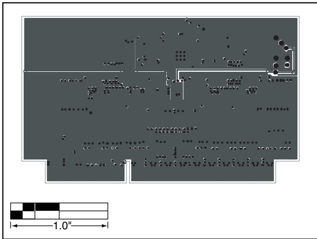
Figure 21. MAX5037 EV Kit PC Board Layout—Inner Layer 2
