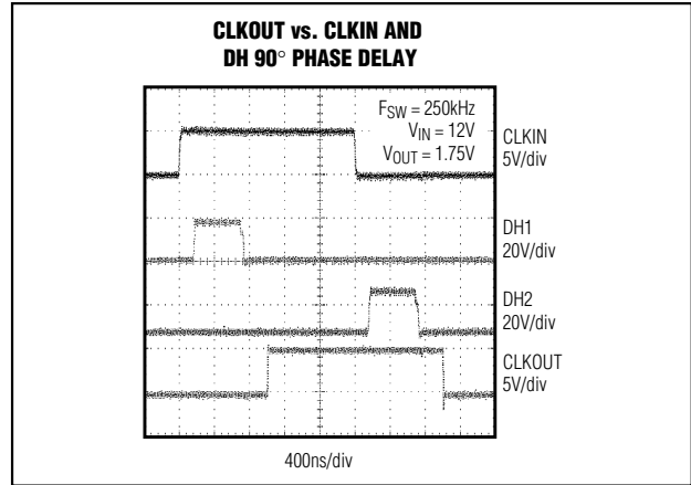
Figure 16. CLKOUT vs. CLKIN and DH 90° Phase Delay
