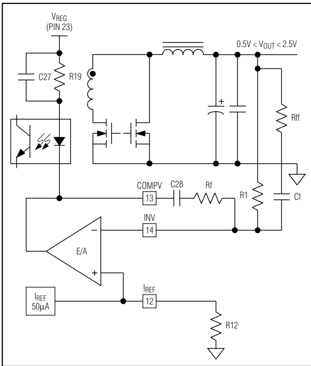
Figure 9. Optocoupler Connection for V_{OUT} < 2.5V
