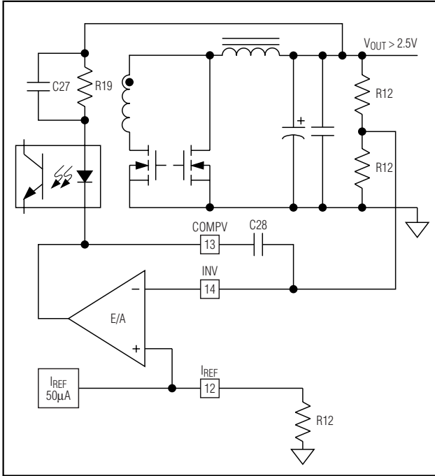
Figure 8. Optocoupler Connection for V_{OUT} > 2.5V
