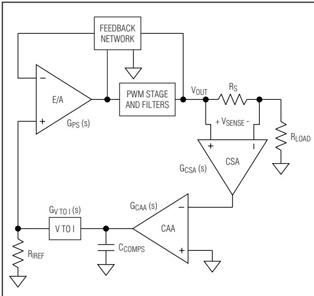
Figure 15. Small-Signal Equivalent Current-Share Control Loop
