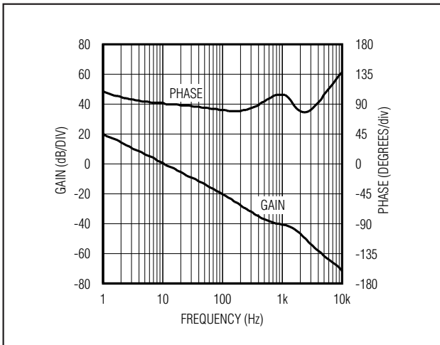
Figure 17. Overall Open-Loop Response of the Current-Share Loop
