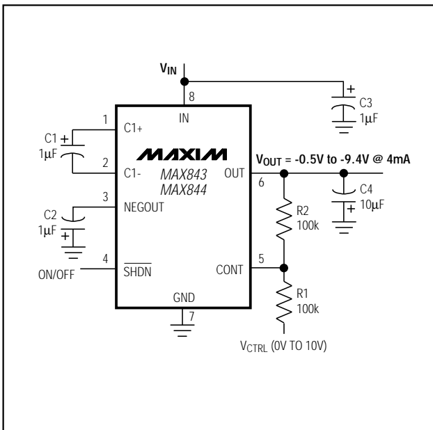
Figure 2c. MAX843/MAX844 Standard Application Circuit
