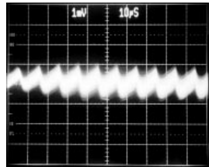
10 \mu s/div V_{IN} = 3.6V , V_{OUT} = -2V , I_{OUT} = 4mA , AC COUPLED
