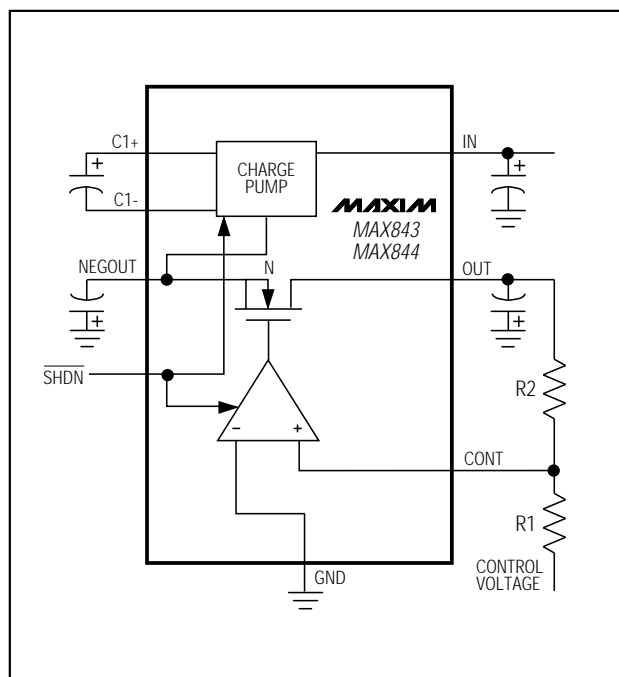
Figure 1b. MAX843/MAX844 Block Diagram
