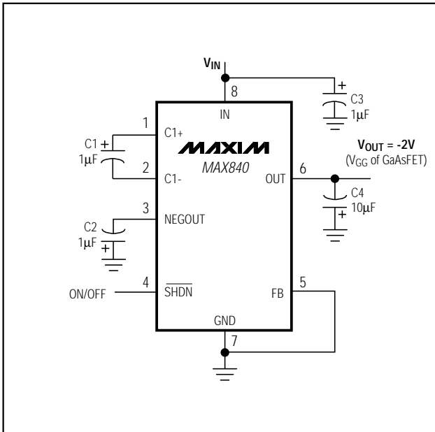
Figure 2a. MAX840 Standard Application Circuit
