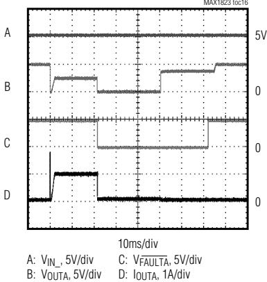
SHORT-CIRCUIT RESPONSE INTO 0Ω (MAX1823A/MAX1823B)
