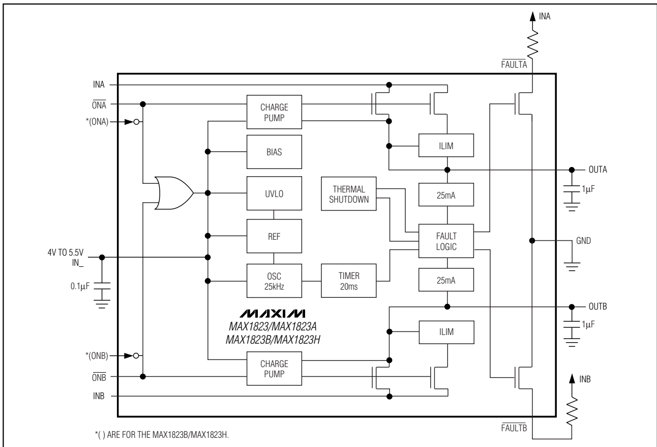
Figure 2. Functional Diagram
