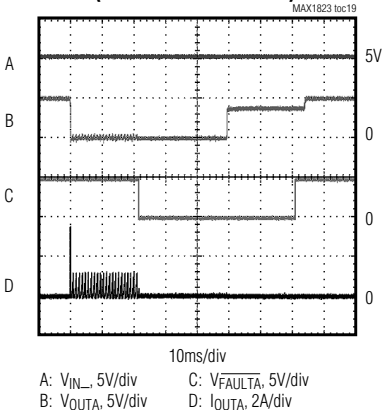
SHORT-CIRCUIT RESPONSE INTO 0Ω (MAX1823A/MAX1823B)
