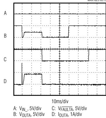
SHORT-CIRCUIT RESPONSE INTO 0Ω (MAX1823/MAX1823H)
