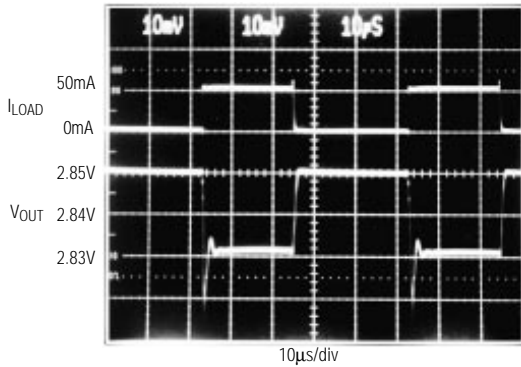
LOAD-TRANSIENT RESPONSE
