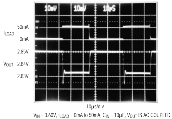
LOAD-TRANSIENT RESPONSE
