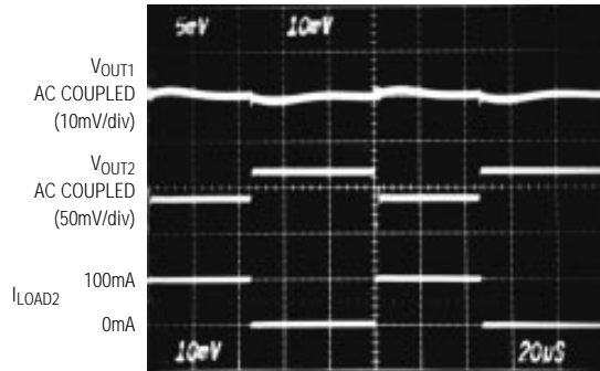
CROSSTALK DUE TO LOAD TRANSIENT
