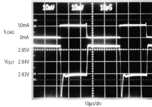
LOAD-TRANSIENT RESPONSE
