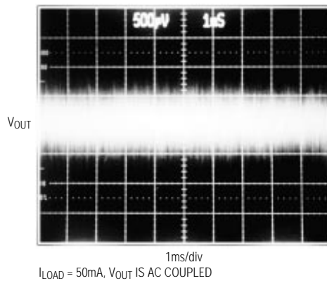
OUTPUT NOISE DC TO 1MHz
