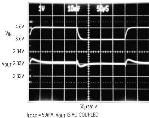
LINE-TRANSIENT RESPONSE
