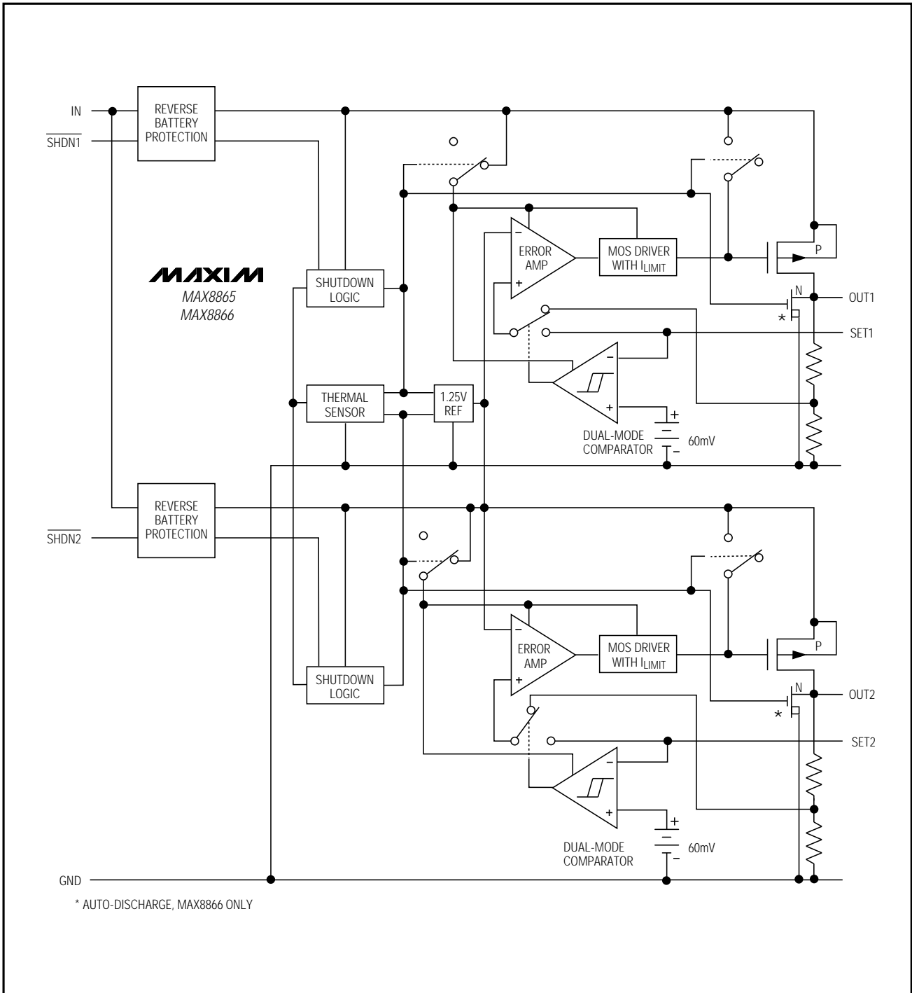
Figure 1. Functional Diagram
