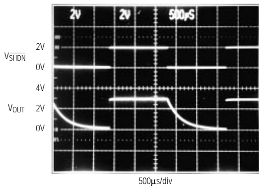
MAX8866 SHUTDOWN (NO LOAD)
