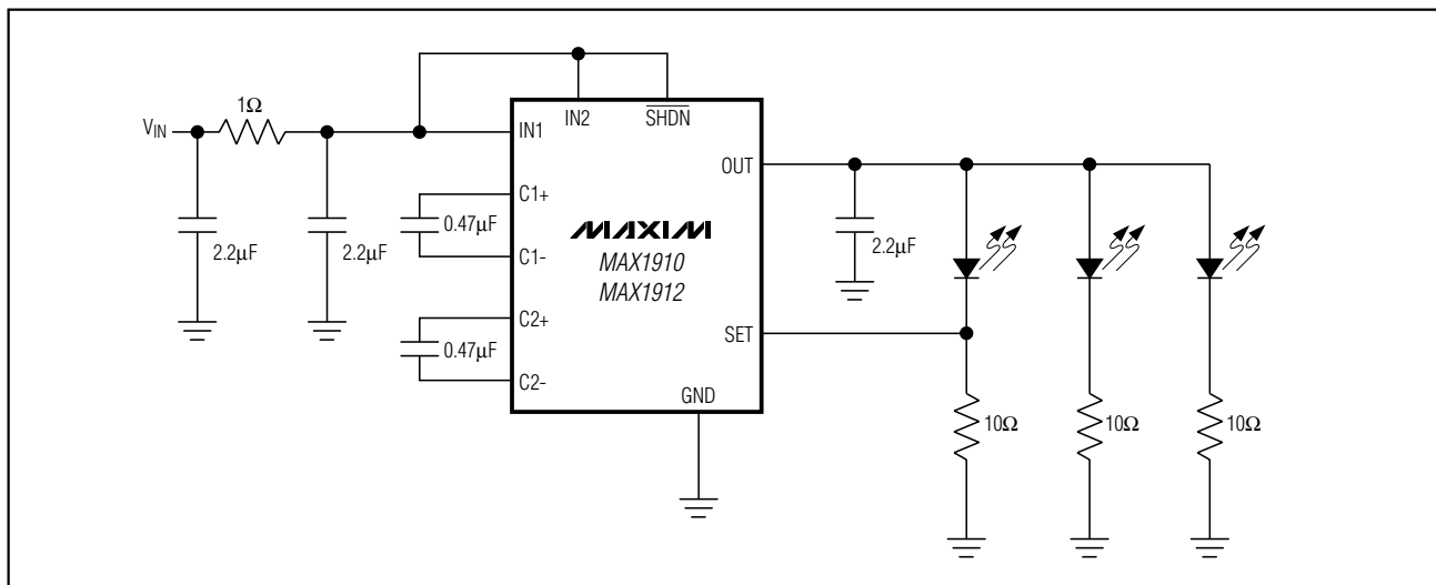
Figure 7. C-R-C Filter Reduces Ripple On the Input
