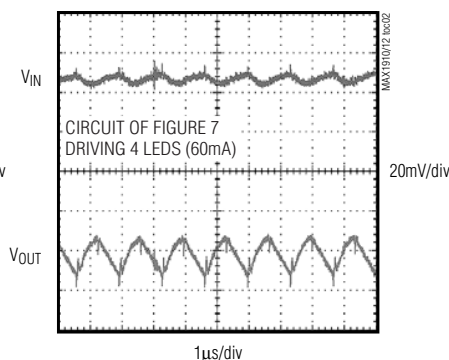
INPUT AND OUTPUT VOLTAGE RIPPLE
