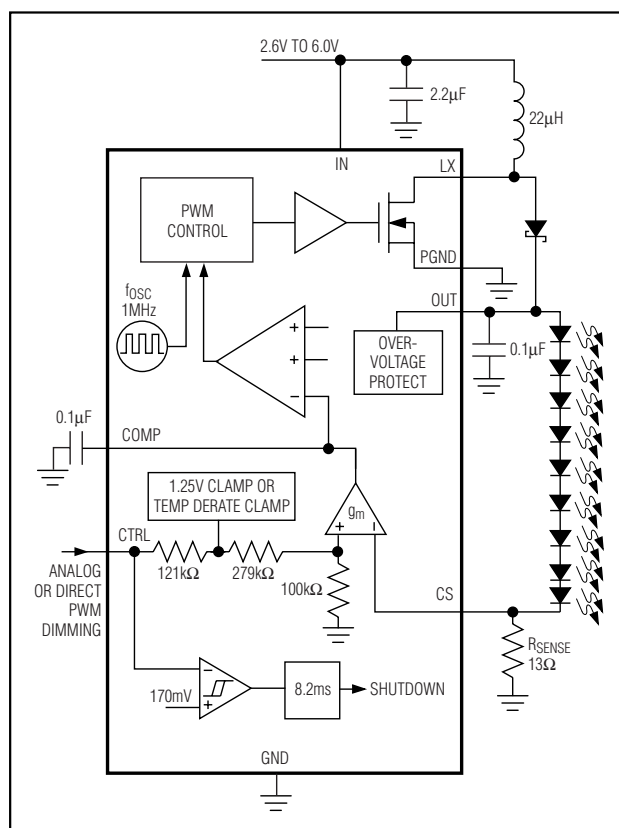
Figure 1. Functional Diagram and Typical Application Circuit
