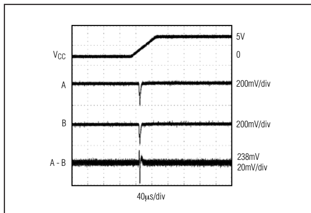
Figure 12. Differential Power-Up Glitch (0.1V/μs)
