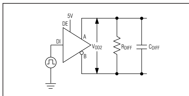
Figure 3. Driver Timing Test Circuit
