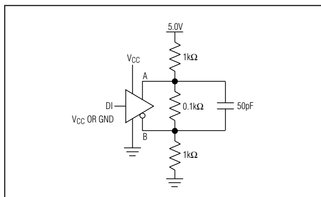
Figure 11. Typical Offset Termination
