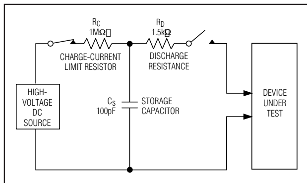
Figure 15a. Human Body ESD Test Model
