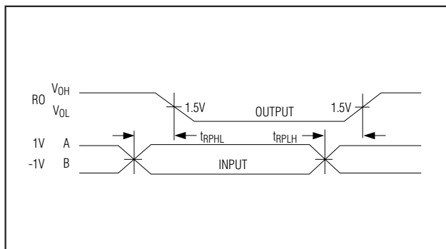
Figure 7. Receiver Propagation Delays
