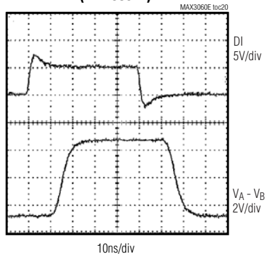
DRIVER PROPAGATION DELAY (MAX3061E)
