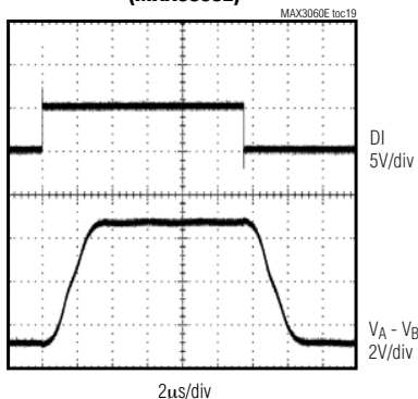
DRIVER PROPAGATION DELAY (MAX3060E)
