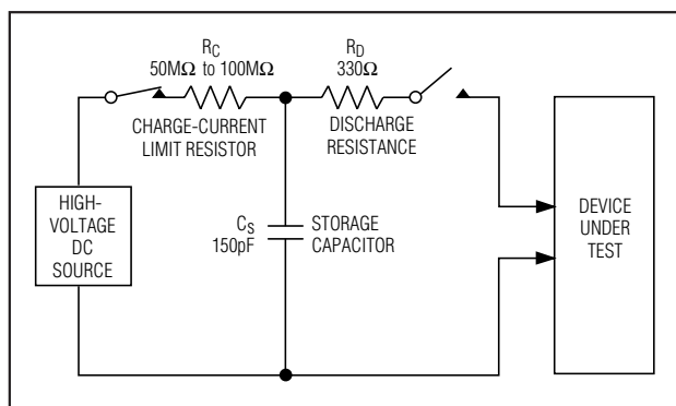
Figure 16. IEC 1000-4-2 ESD Test Model
