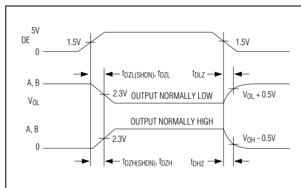
Figure 6. Driver Enable and Disable Times
