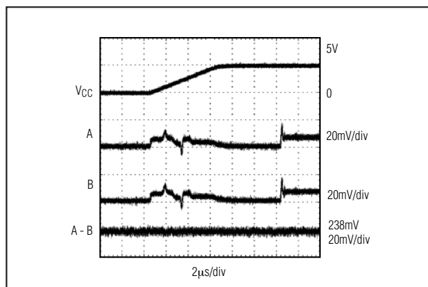
Figure 13. Differential Power-Up Glitch (1V/μs)
