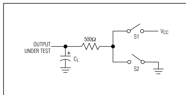
Figure 4. Driver Enable/Disable Timing Test Load
