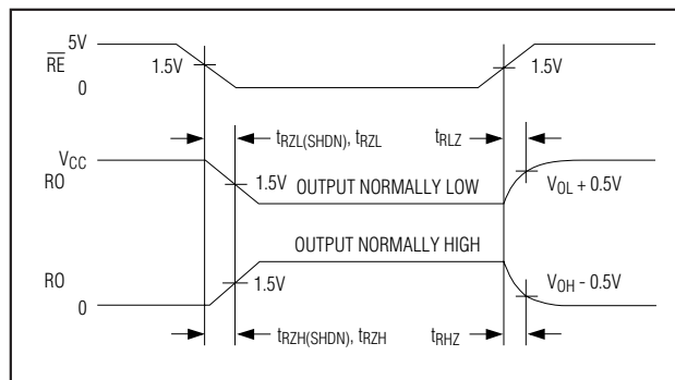
Figure 8. Receiver Enable and Disable Times
