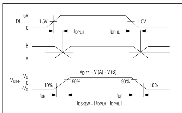
Figure 5. Driver Propagation Delays
