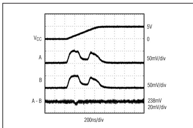
Figure 14. Differential Power-Up Glitch (10V/μs)
