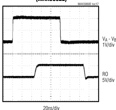
RECEIVER PROPAGATION DELAY (MAX3062E)
