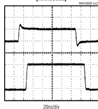
DRIVER PROPAGATION DELAY (MAX3062E)
