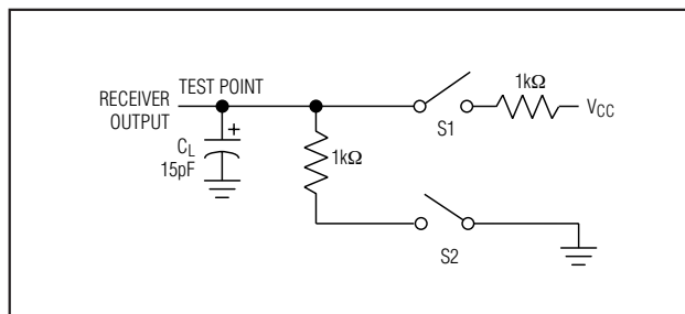
Figure 2. Receiver Enable/Disable Timing Test Load
