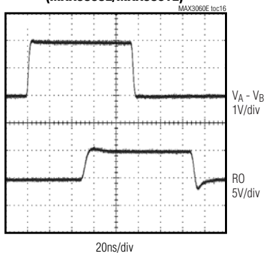
RECEIVER PROPAGATION DELAY (MAX3060E/MAX3061E)
