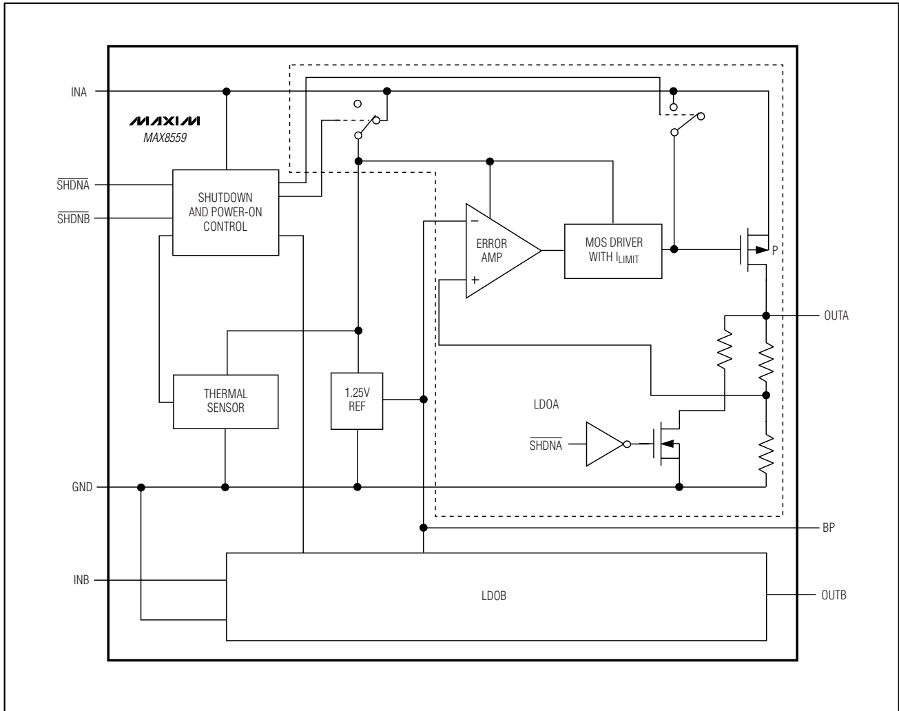
Functional Diagram
