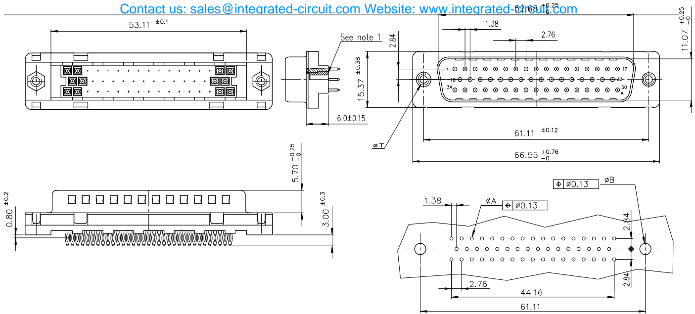
PC board drilling dimensions (after plating - thickness: 1.60 to 3.20 mm)
