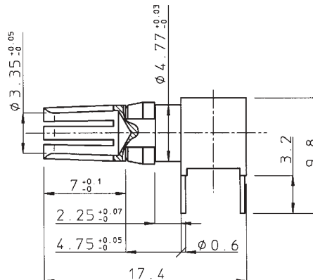
socket contact
