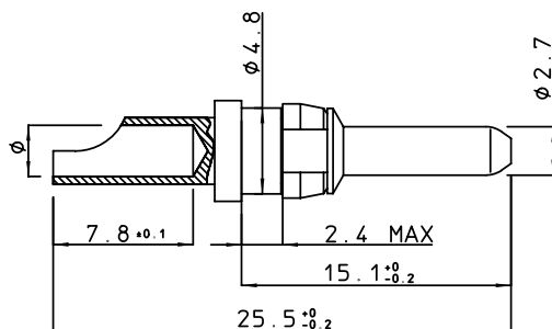
pin contact
