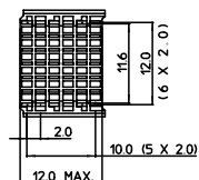
HM2H42P1□□ (type 6X5)
