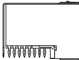
HM2R88PA8108N9 (top shielded only, 4 mm pitch)
