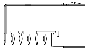
HM2R02PA5108N9 (top shielded only, 4 mm pitch)
