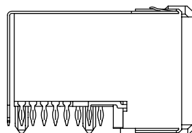
HM2R82PA8108N9 (top shielded only, 4 mm pitch)
