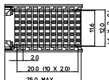
HM2H80P1□□ (type CR)
