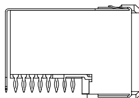
HM2R90PA8108N9 (top shielded only, 4 mm pitch)
