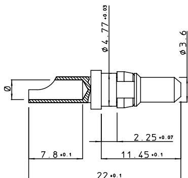
pin contact
