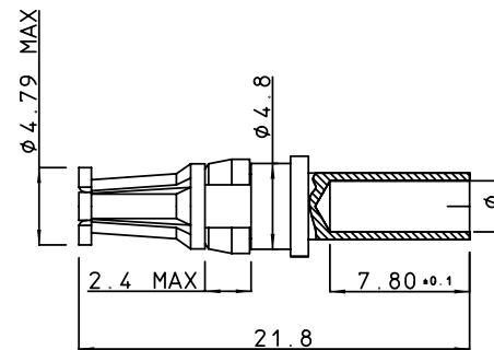
socket contact
