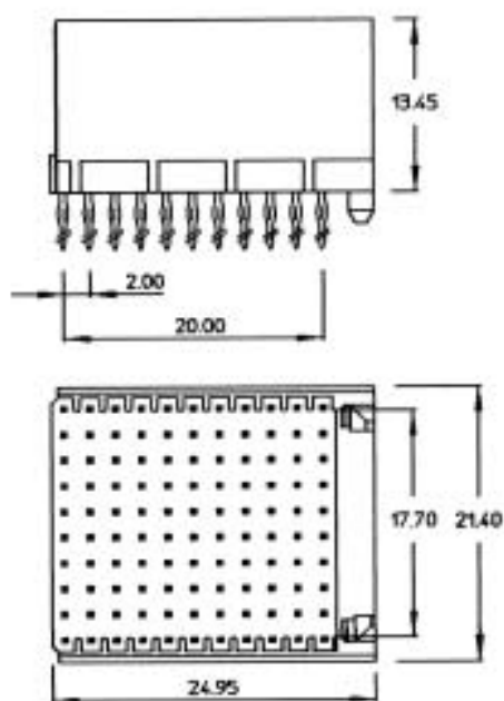
Standard loading patterns (seen from mating side)
