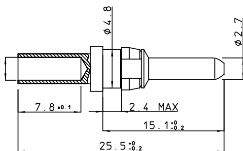
pin contact
