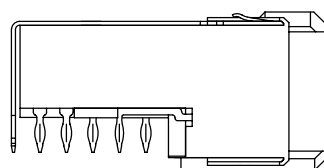
HM2R10PA5108N9 (top shielded only, 4 mm pitch)
