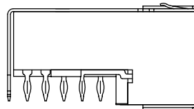
HM2R71PA5108N9 (top shielded only, 4 mm pitch)
