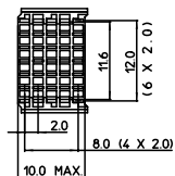
HM2H06P1□□ (type 5X5)
