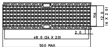
HM2H65P1□□ (type AB)
