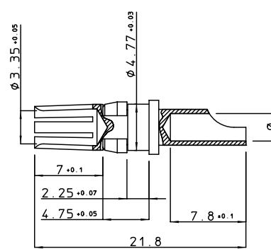
socket contact
