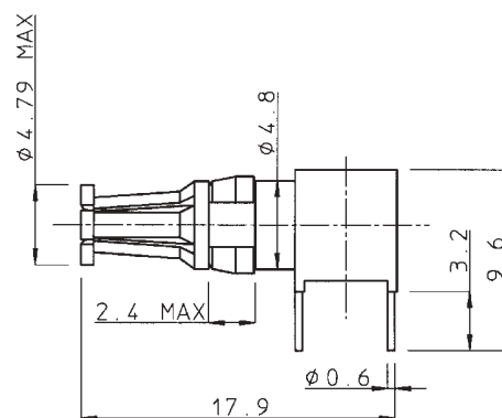
socket contact
