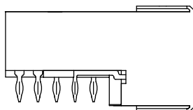
HM2R71PA5100N9 (non shielded)
