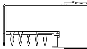
HM2R70PA5108N9 (top shielded only, 4 mm pitch)
