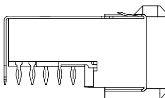
HM2R67PA5108N9 (top shielded only, 4 mm pitch)
