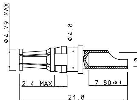
socket contact
