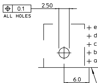
PCB-HOLE LAYOUT COMPONENT SIDE
