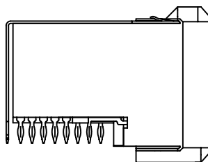
HM2R95PA8108N9 (top shielded only, 4 mm pitch)
