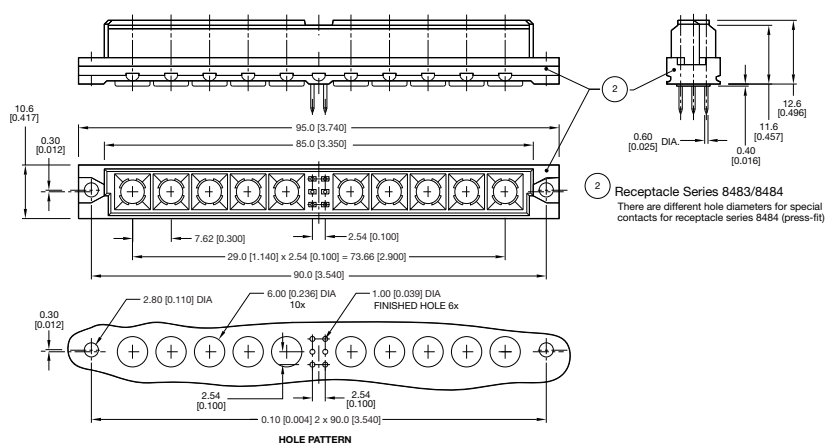
CONTACT ARRANGEMENT
