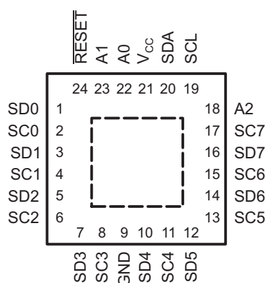
RGE PACKAGE (TOP VIEW)
