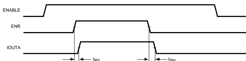
Figure 3. Read Timing
