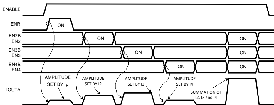
Figure 1. Functional Timing Diagram
