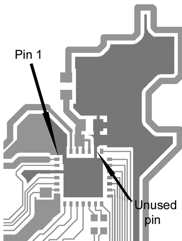
Figure 16. Heat Sinking
