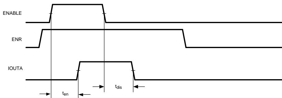
Figure 2. Enable Timing
