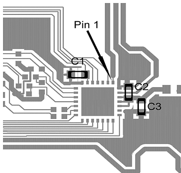
Figure 15. Decoupling Capacitors
