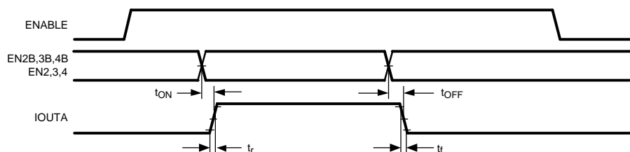
Figure 4. Write Timing
