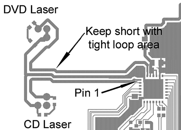
Figure 14. Laser Connection
