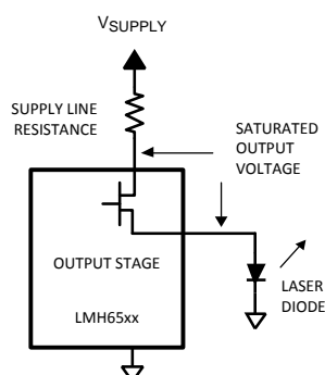
Figure 12. Output Configuration
