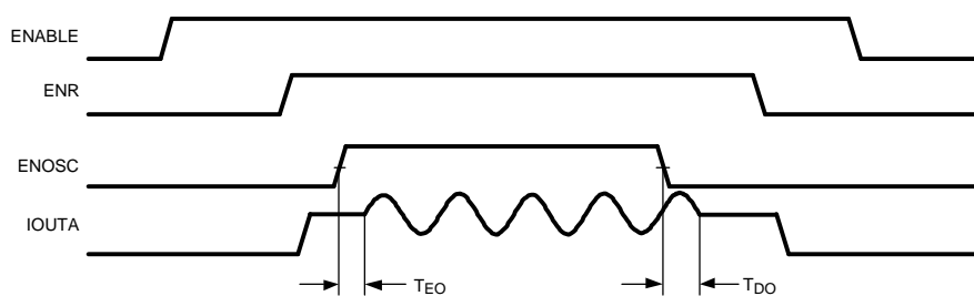
Figure 5. Oscillator Timing
