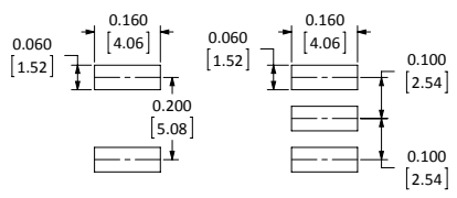
BOTTOM TOP RECOMMENDED FOOTPRINT
