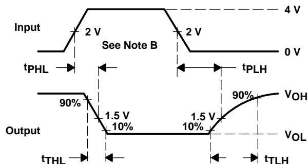
VOLTAGE WAVEFORMS
