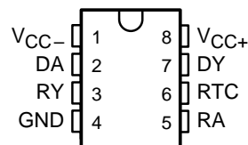
P OR PS PACKAGE TOP VIEW
