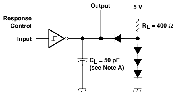
TEST CIRCUIT
