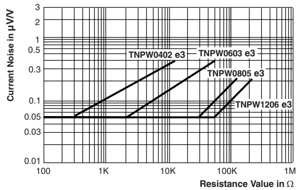
Current Noise
