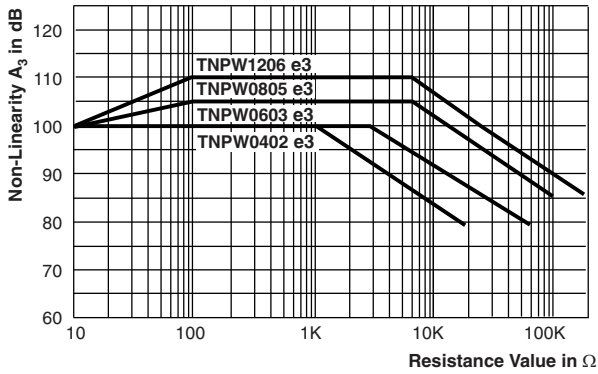
Non-Linearity
