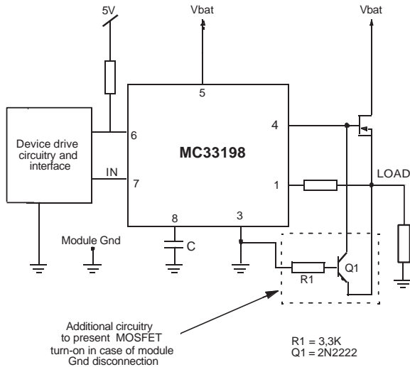
Figure 19. 33198 GND Disconnection Circuitry
