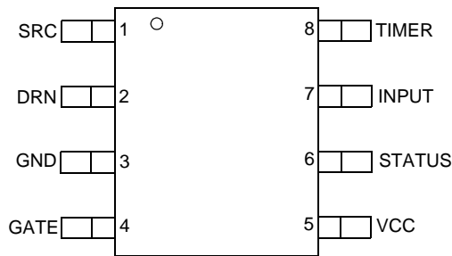
Figure 3. 33198 Pin Connections
