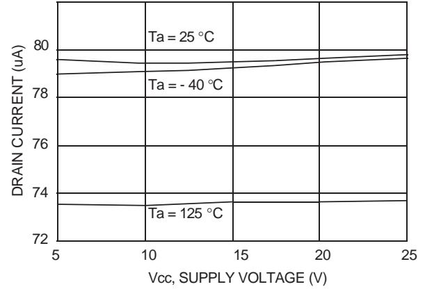
Figure 9. Drain Current versus Supply Voltage
