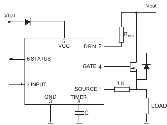
Figure 18. 33198 Reverse Battery
