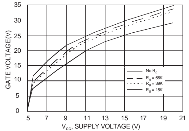
Figure 15. Gate Voltage versus VCC and RG at TA = 25°C
