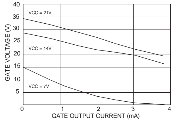
Figure 14. Gate Voltage versus Gate Output Current. TA = 40°C
