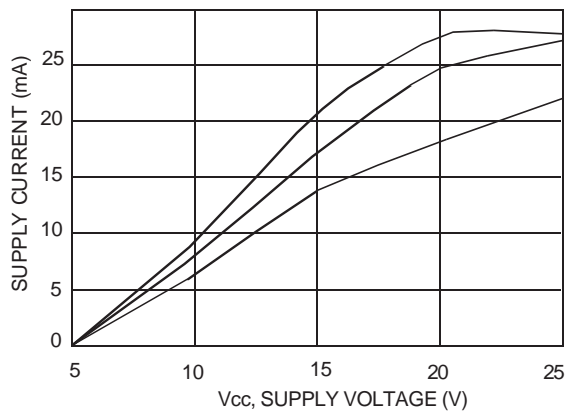
Figure 7. Supply Current versus Supply Voltage. Pin 7 = 5.0V
