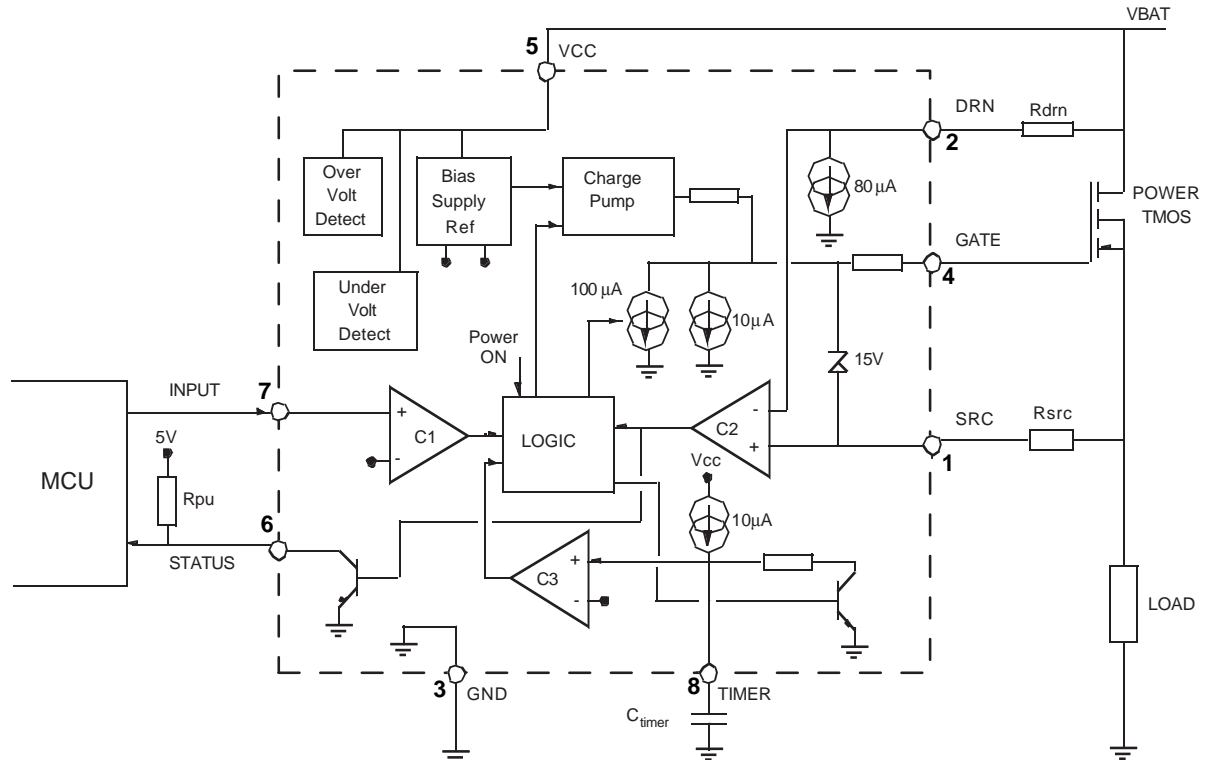
Figure 2. 33198 Simplified Internal Block Diagram and Typical Application
