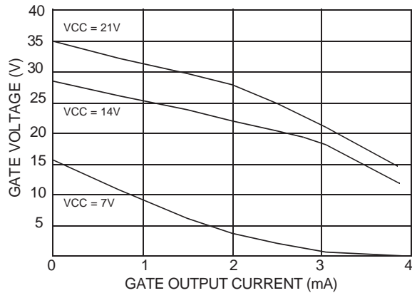
Figure 12. Gate Voltage versus Gate Output Current. TA = 25°C.
