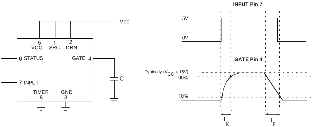
Figure 4. Timing Measurements Test Schematic
