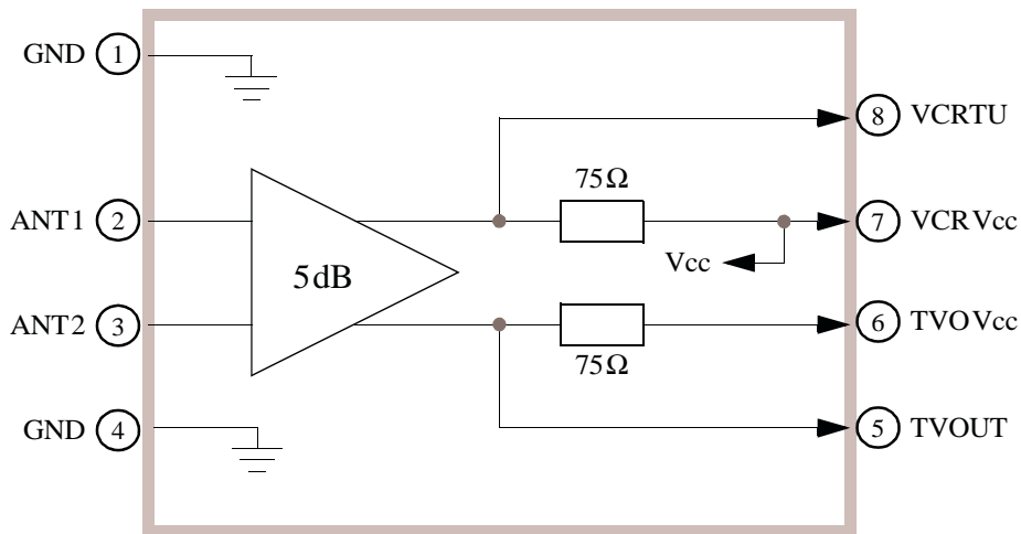
Figure 2. Simplified Block Diagram—MC44BC380
