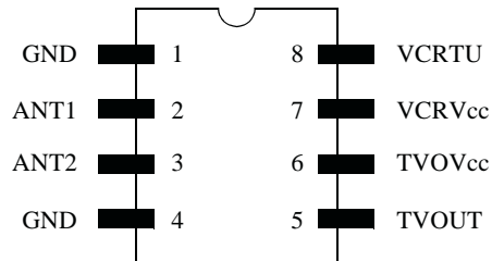
Figure 1. Pin Connections
