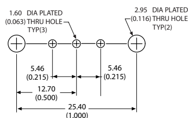
Recommended hole pattern for 8241-CL11G
