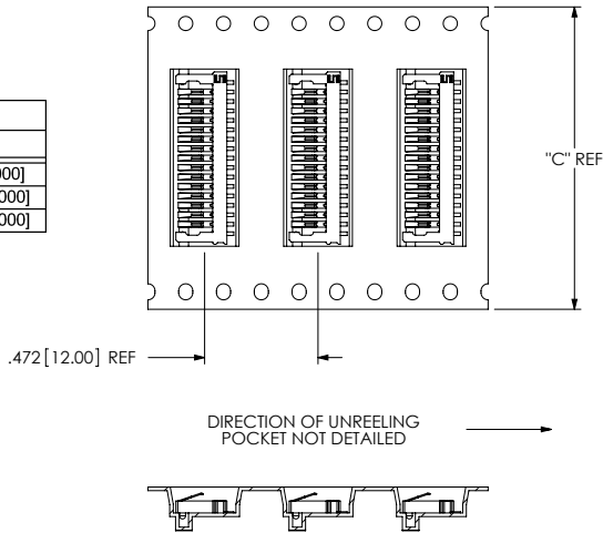
PACKAGING VIEW (SEL-115-02-XXX-S-TR SHOWN) (SEE NOTE 5)
