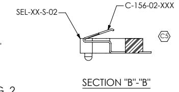
FIG. 2 SEL-115-02-XXX-S SHOWN (DIFFERENT AS SHOWN, OTHERWISE SAME AS -01 LEAD STYLE)
