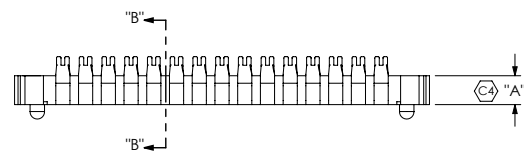
FIG. 2 SEL-115-02-XXX-S SHOWN (DIFFERENT AS SHOWN, OTHERWISE SAME AS -01 LEAD STYLE)
