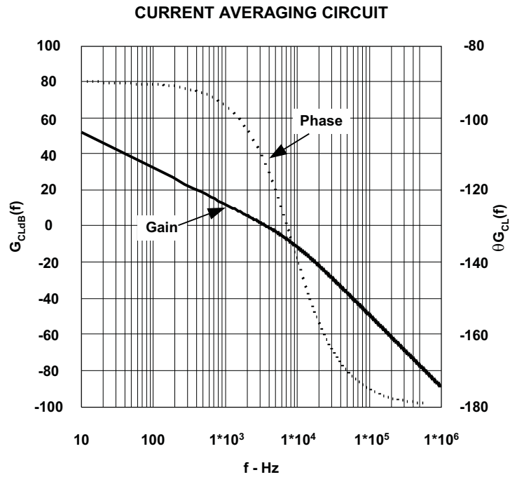
Figure 30. Bode Plot of the Current Averaging Circuit.
