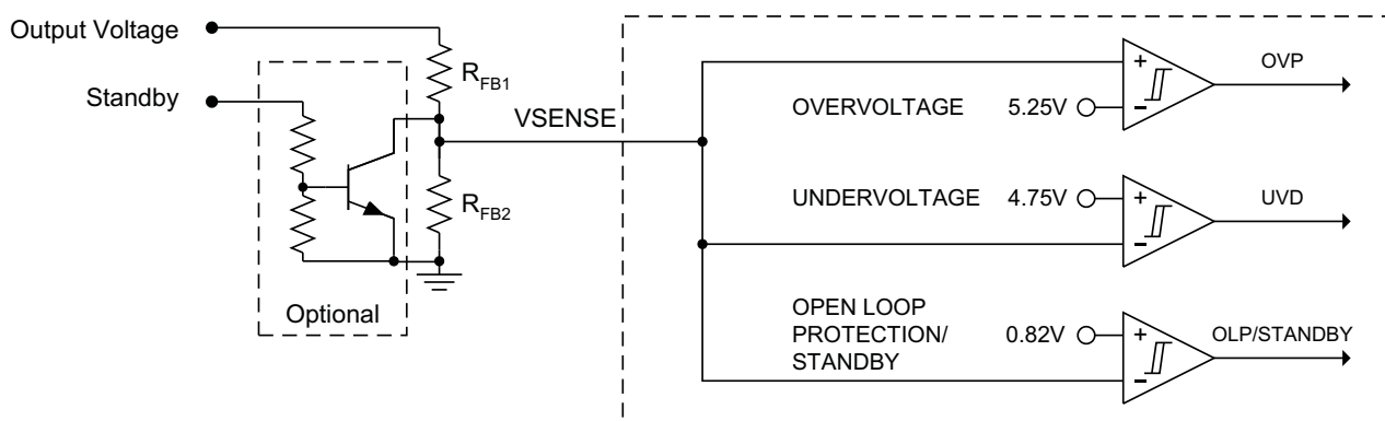
Figure 24. Over Voltage Protection, Open Loop Protection/Standby
