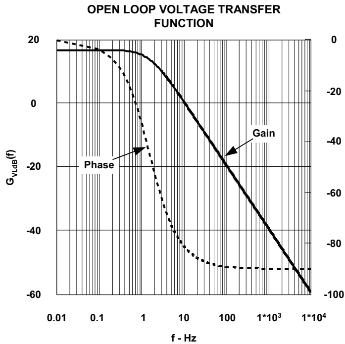
Figure 31. Bode Plot of the Open Loop Voltage Transfer Function
