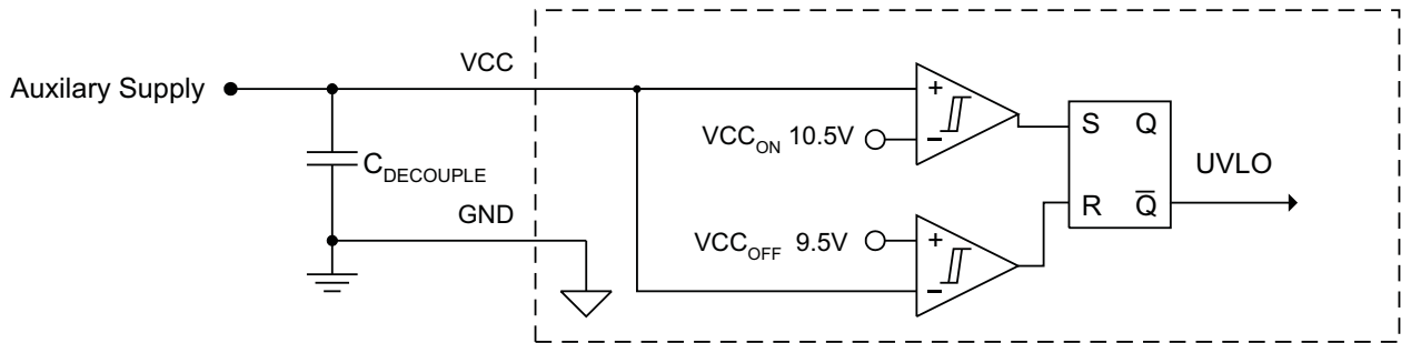
Figure 22. UVLO
