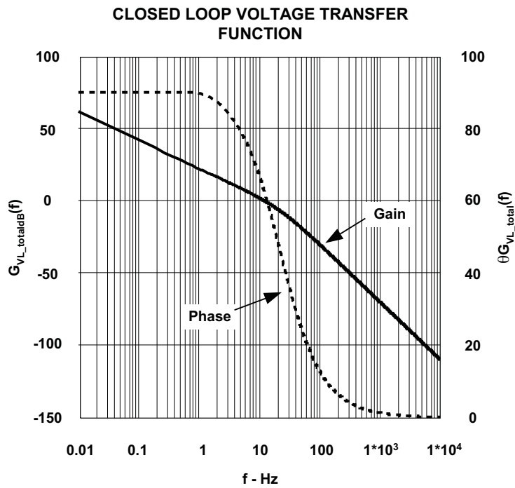
Figure 32. Closed Loop Voltage Bode Plot
