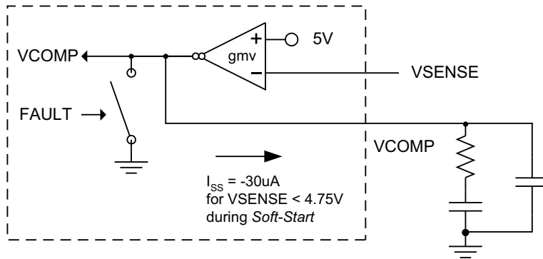
Figure 20. Soft Start
