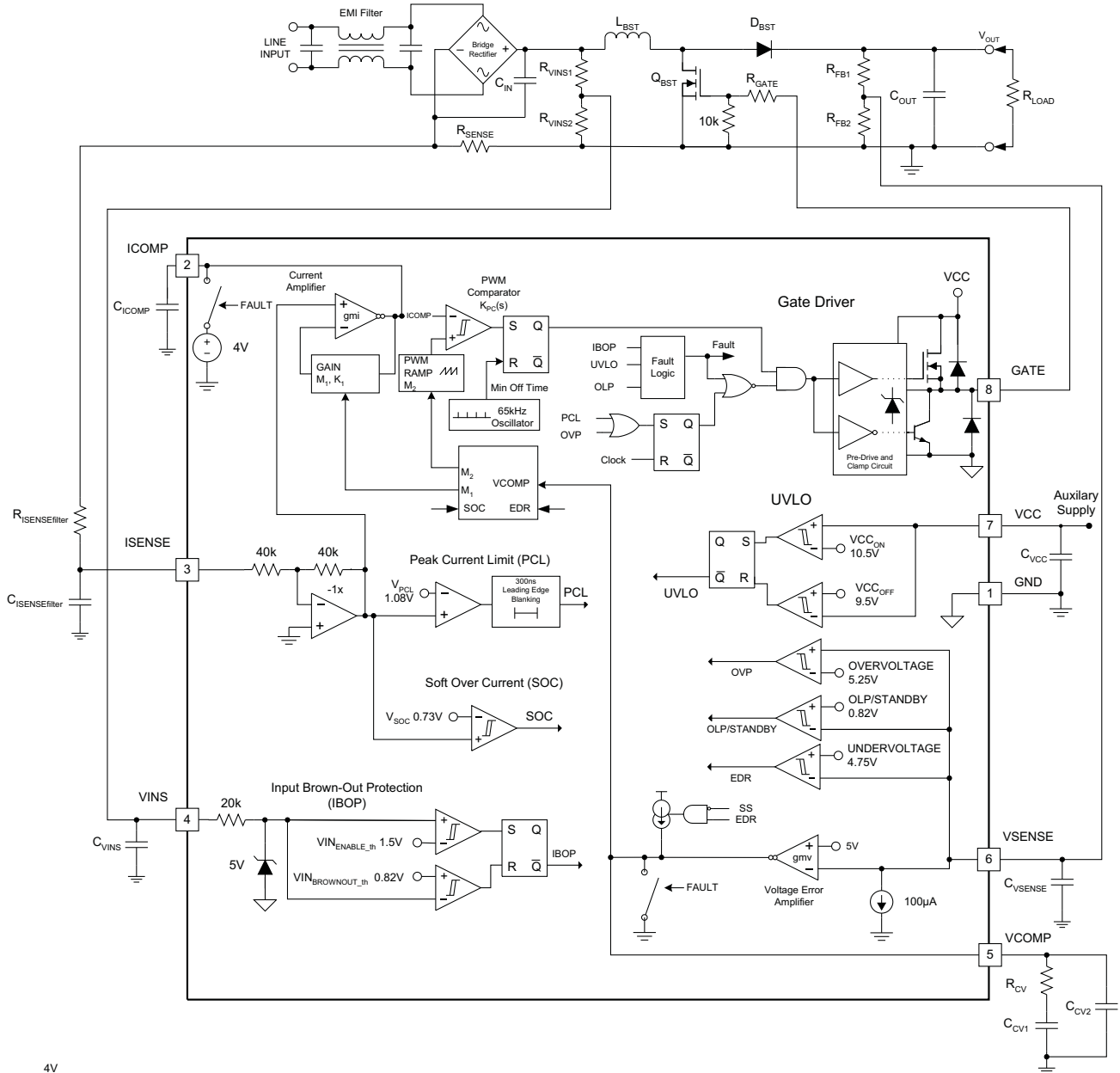
Figure 18. Block Diagram
