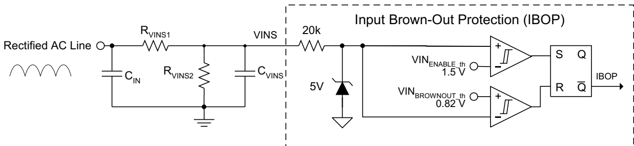
Figure 23. Input Brown-Out Protection (IBOP)
