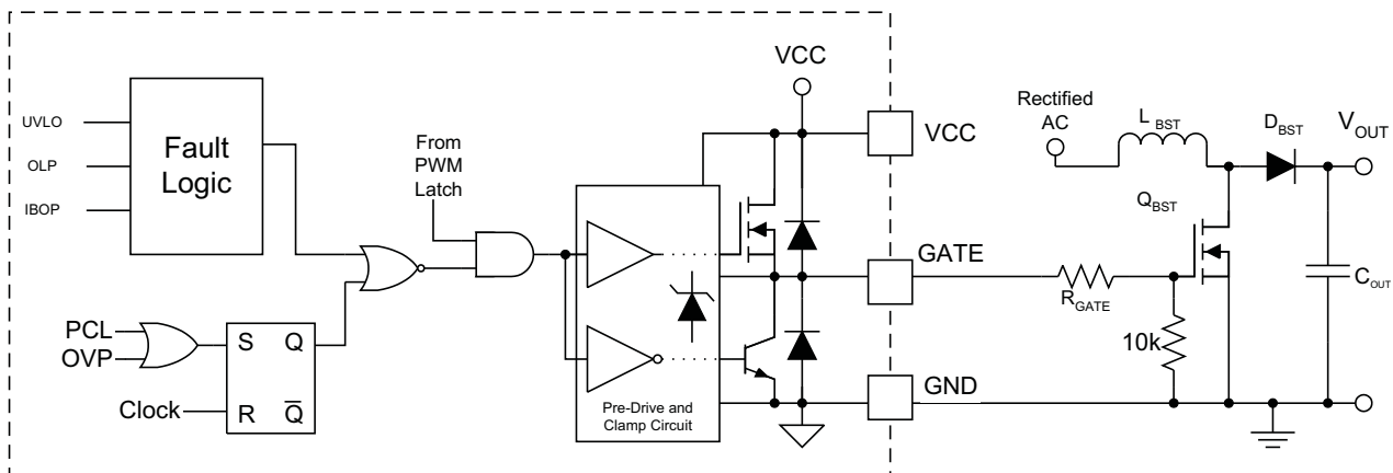
Figure 26. Gate Driver
