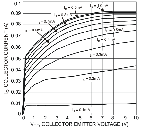
Fig. 4 Typical Collector Current vs. Collector Emitter Voltage
