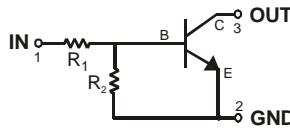
Device Symbol
