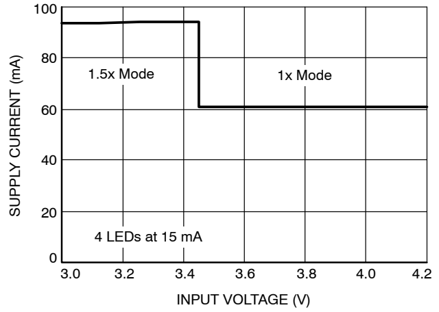
Figure 10. Supply Current vs. Input Voltage
