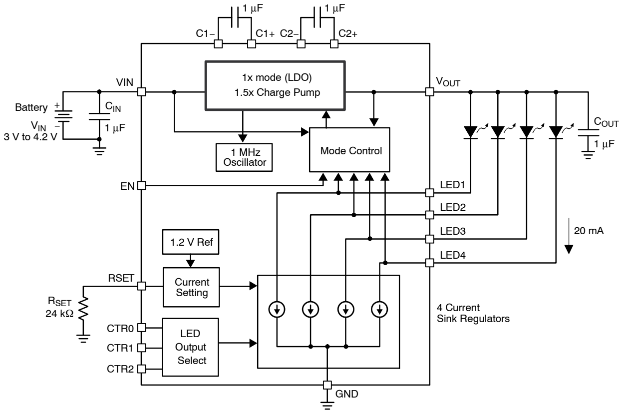
Figure 2. CAT3604 Functional Block Diagram
