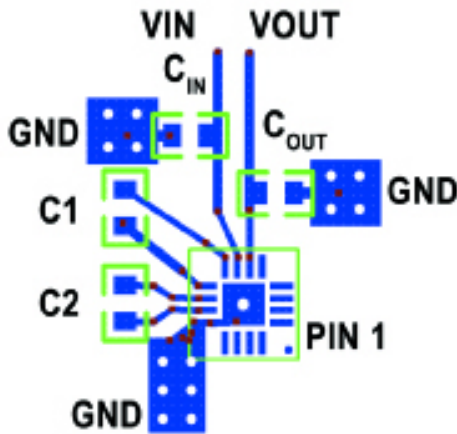
Figure 22. PCB Layout
