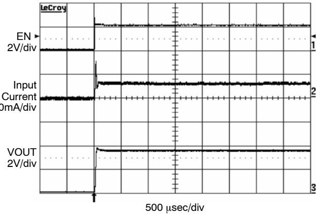
Figure 18. Power Up 4 LEDs at 15 mA, V_{in} = 3.6\text{ V} (1x Mode)
