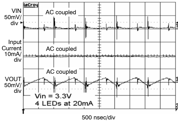
Figure 15. Switching Waveforms in 1.5x Mode
