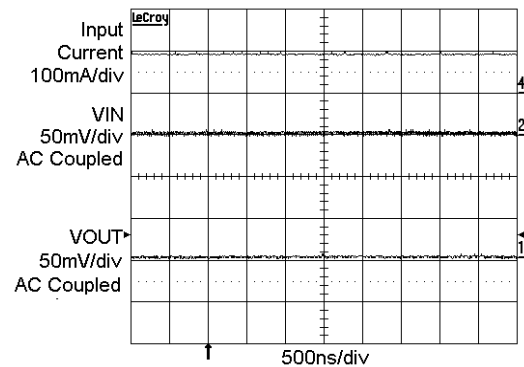
Figure 20. Operating Waveforms in 1x Mode
