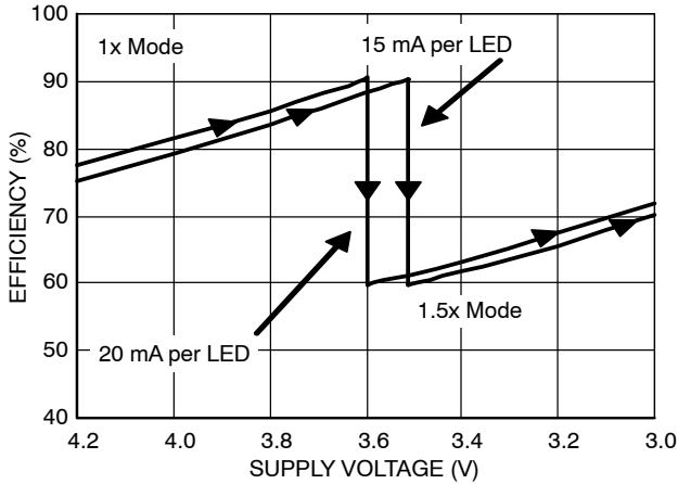
Figure 3. Efficiency vs. Supply Voltage (6 LEDs)
