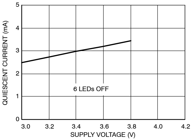
Figure 7. Quiescent Current vs. Supply Voltage (1.5x Mode)
