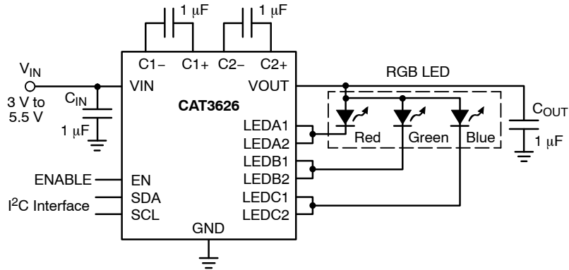
Figure 29. RGB LED
