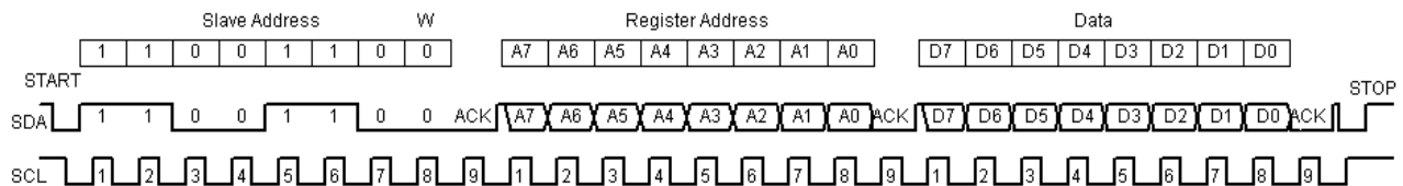
Figure 26. Write Instruction Sequence
