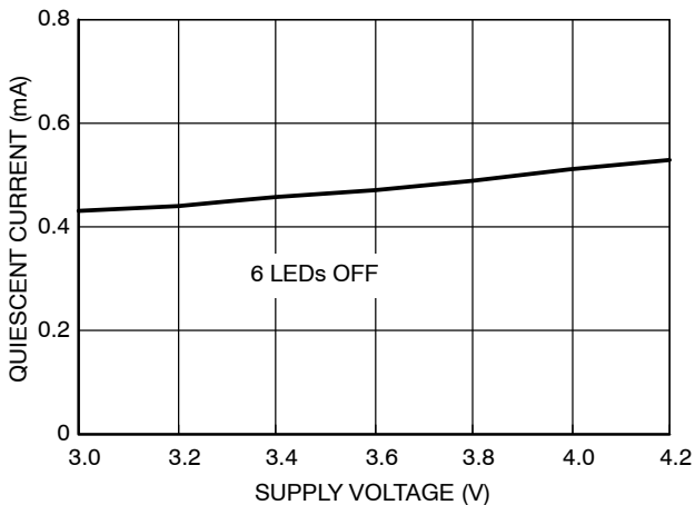
Figure 5. Quiescent Current vs. Supply Voltage (1x Mode)
