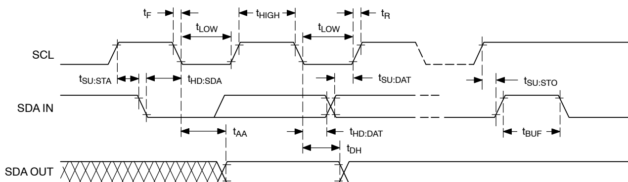
Figure 2. I 2 C Bus Timing Characteristics
