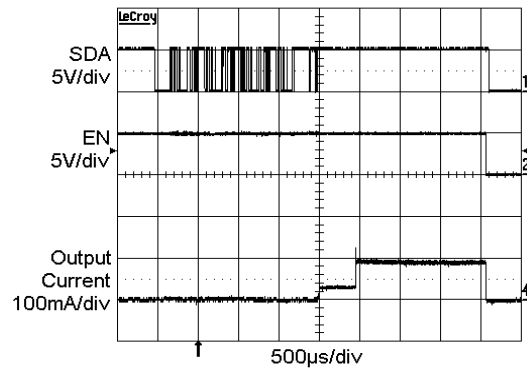
Figure 18. Enable Power Down (1.5x Mode)
